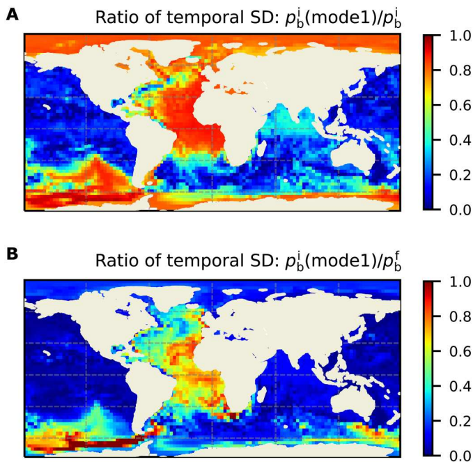
Fig. 2. Importance of mode 1 p_b^i variability. Ratio of the temporal SD of the mode 1 p_b^i to that of total p_b^i (A) and of p_b^f (B) using one arbitrary ensemble member.
