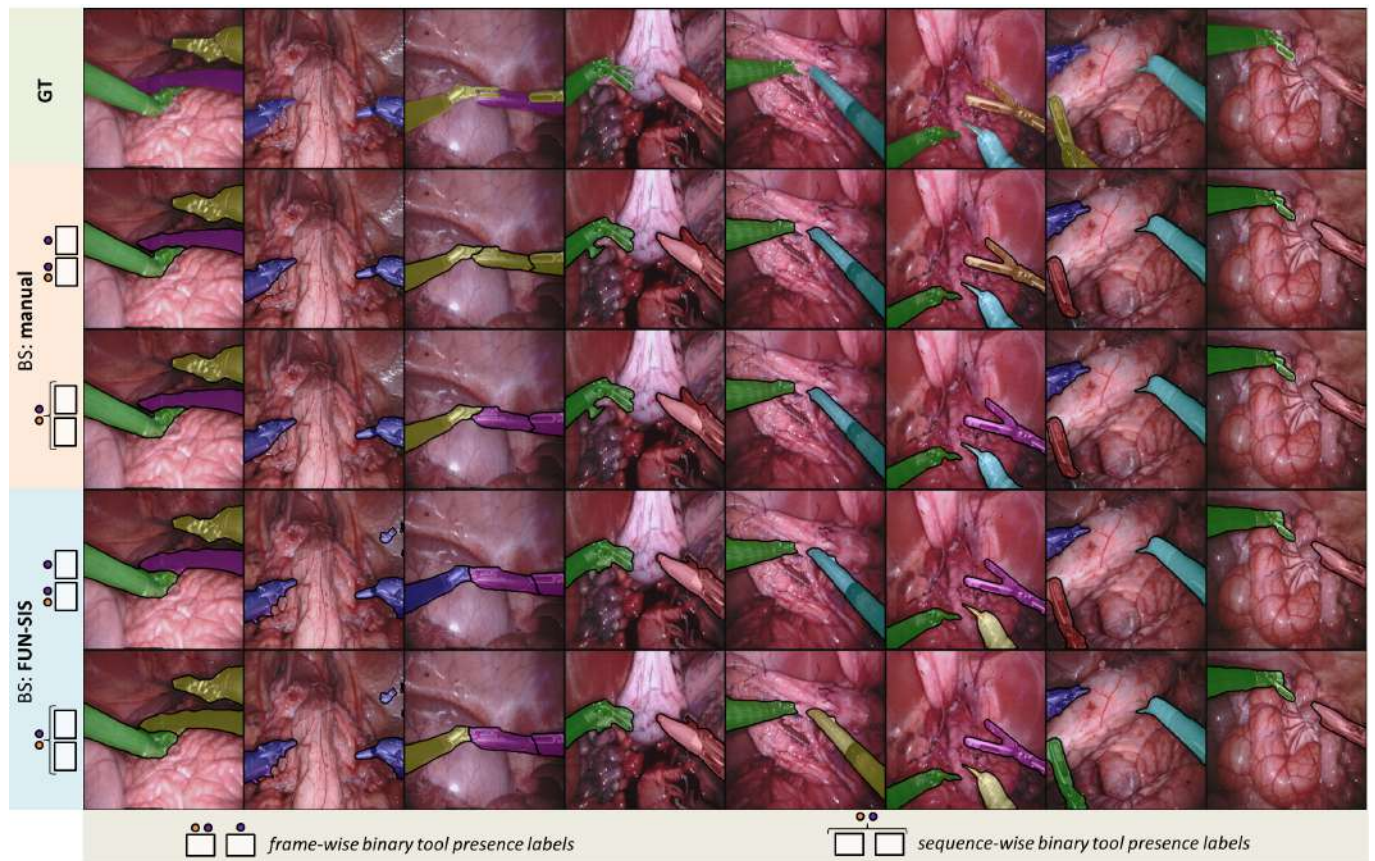
Fig. 12: Qualitative segmentation results from the EndoVis2017 dataset, highlighting, for our SAF-IS approach, the source of binary segmentation masks (BS) and the type of binary tool presence labels (frame-wise or sequence-wise). All the SAF-IS results are obtained using 8 prototype labels. Row 1: ground truth; rows 2-5: SAF-IS Student trained on (2) manually annotated binary masks and frame-wise tool presence labels, (3) manually annotated binary masks and sequence-wise tool presence labels, (4) FUN-SIS predicted binary masks and frame-wise tool presence labels, (3) FUN-SIS predicted binary masks and sequence-wise tool presence labels.
