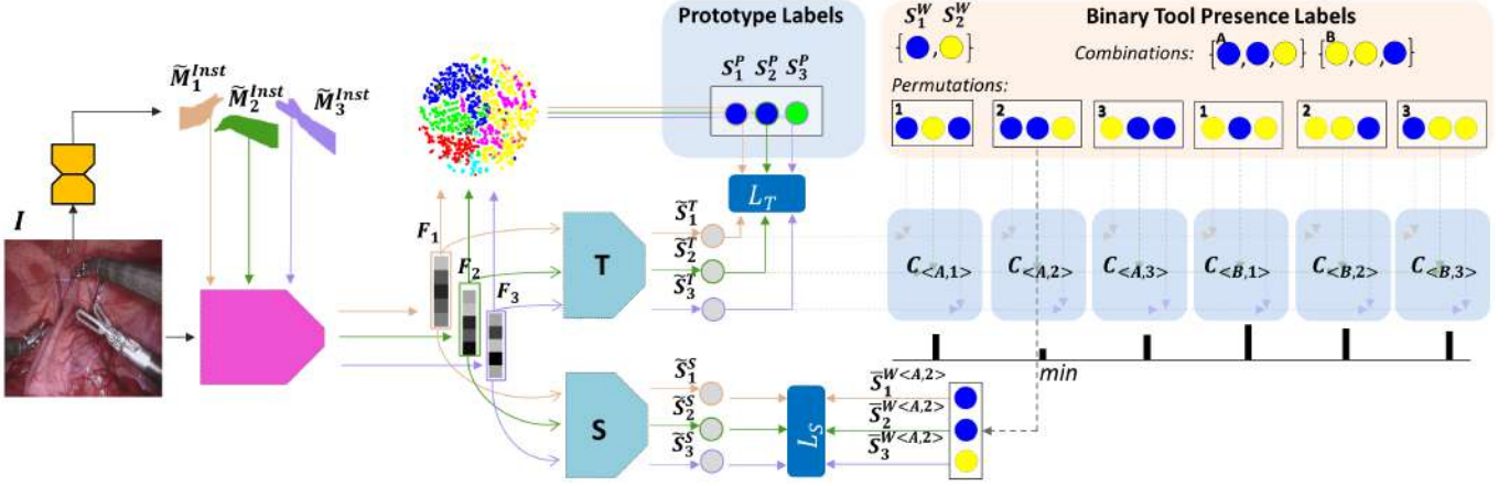
Fig. 7: Overview of the proposed weakly-supervised instance classification module. Given an image I , the corresponding set of instance-wise features \{F_i\} , with i in [1, \tilde{N}_{Inst}] , is obtained from the instance masks \tilde{M}_i^{Inst} . Each feature is mapped to the corresponding prototype label S_i^P , which, as shown in this case, does not necessarily correspond to the ground truth label. Each feature is also independently passed through the Teacher (T) and Student networks (S), yielding the predicted probabilities \tilde{P}_i^T , \tilde{P}_i^S , and the corresponding predicted labels \tilde{S}_i^T , \tilde{S}_i^S (for the sake of readability only the latter are shown in the picture). T is trained optimizing the loss L_T computed using the prototype labels \{S_i^P\} . Simultaneously, T predictions are used to compute the assignment costs C_{(i_c, i_p)} for each i_p permutation of each i_c combination of the weak labels \{S_i^W\} , with i in [1, N_W] . The ordered set \{\tilde{S}_i^S\} , with i in [1, \tilde{N}_{Inst}] , corresponding to the minimum assignment cost, is used to compute the loss L_S for Student network optimization.
