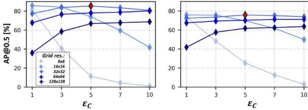
Fig. 8: Impact of grid square resolution and threshold value \epsilon_C on the tool instantiation quality for the EndoVis2017 dataset (left) and EndoVis2018 dataset (right). The combination used in our main experiments is highlighted in red.
