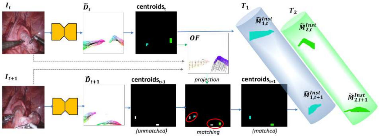
Fig. 5: Overview of the tracking strategy used to generate positive samples for contrastive learning. Given two consecutive frames, the centroids at time t , obtained from the displacement field D_t , are mapped to the I_{t+1} space using optical flow OF , computed between the two images I_t and I_{t+1} . The projected centroids are then matched to the ones obtained from the displacement field D_{t+1} . This allows building the set of tubes \{T_i\} , with i in [1, \tilde{N}_{Inst}] . Tubes are progressively grown by repeating this process for consecutive frames.
