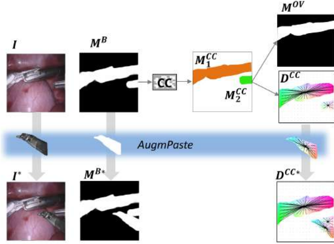
Fig. 3: Overview of the proposed strategy to generate a pseudo-supervision signal to learn instrument instantiation. Given an image I , its binary mask M^B is instantiated using a Connected Component (CC) algorithm, yielding the set of tool masks \{M_i^{CC}\} , with i in [1, N_{CC}] . From them, the displacement field D^{CC} and the overlap mask M^{OV} can be automatically obtained. A random tool instance is then selected from the training set, and pasted on I , M^B , D^{CC} , producing their augmented versions I^* , M^{B*} , D^{CC*} .
