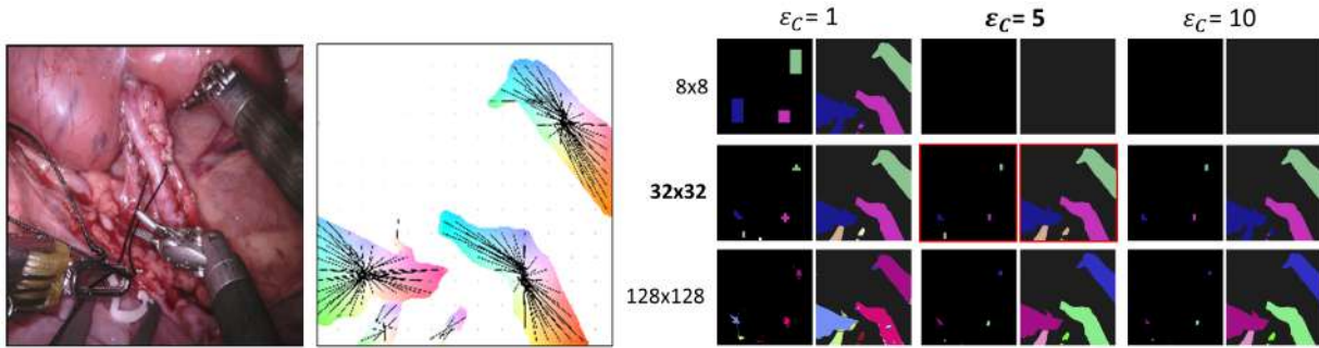
Fig. 9: From left to right, original image, predicted displacement field, and examples of centroid regions and instantiation masks for different combinations of grid resolution and threshold \epsilon_C . Mask colors indicate the ID assigned to the tube each instance belongs to. The combination adopted in our main experiments is highlighted in red.
