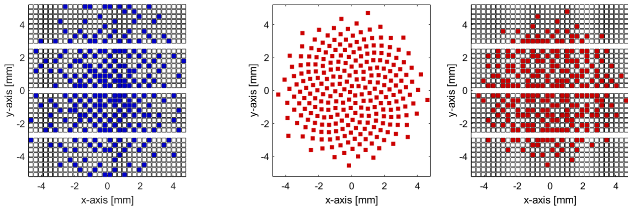
Fig. 4. Layouts of the sparse arrays implemented on the Vernon matrix probe. The layout on the left was obtained through SA optimization and software elements selection [63]. The layout on the right was obtained through hardware selection of the elements closest to the ideal positions of the sunflower seeds (center) [79]–[81].
