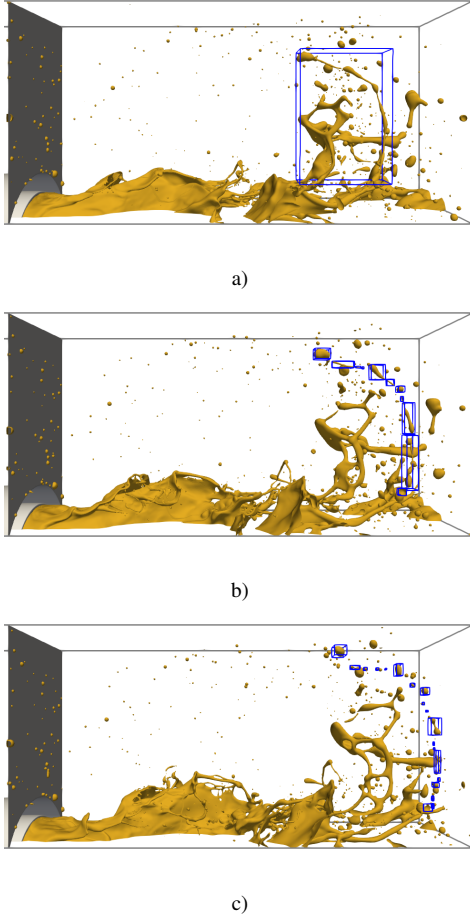
Figure 11: Tracking of structures from a ligament detached from a liquid pocket in three subsequent snapshots.
