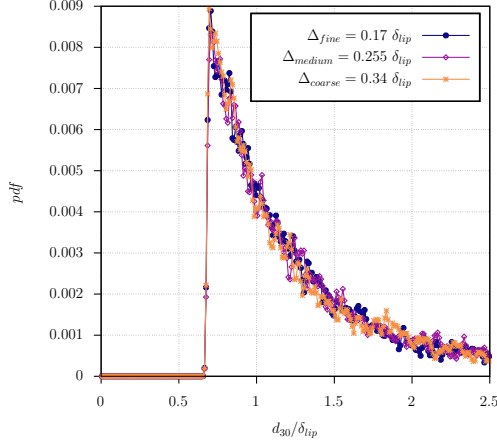
Figure 3: Probability density functions with different mesh resolutions considering droplets bigger than 2\Delta_{coarse} .
