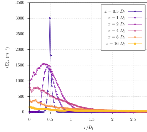
Figure 16: Radial profiles of spatial- and time-averaged interface area density \langle \Sigma \rangle_\theta .
