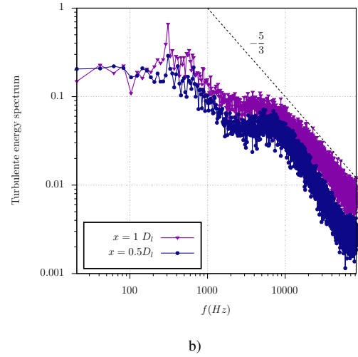
Figure 10: Streamwise velocity spectra on the medium case i.e. \Delta_{medium} = 51 \mu m .
