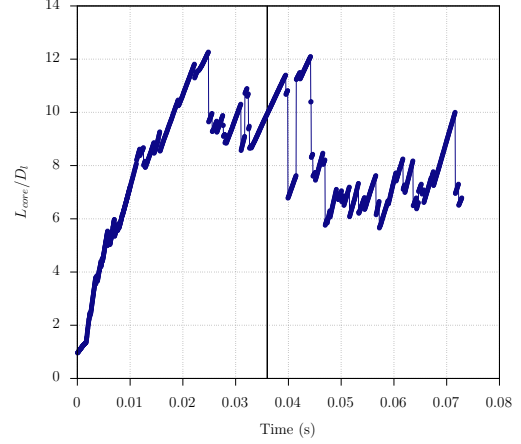
Figure 4: Continuous liquid core length evolution and the estimated transient time (solid vertical line).
