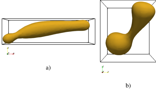
Figure 14: Examples of ligaments in different configurations: a) aligned in the direction of the mesh, b) diagonal to the mesh directions.
