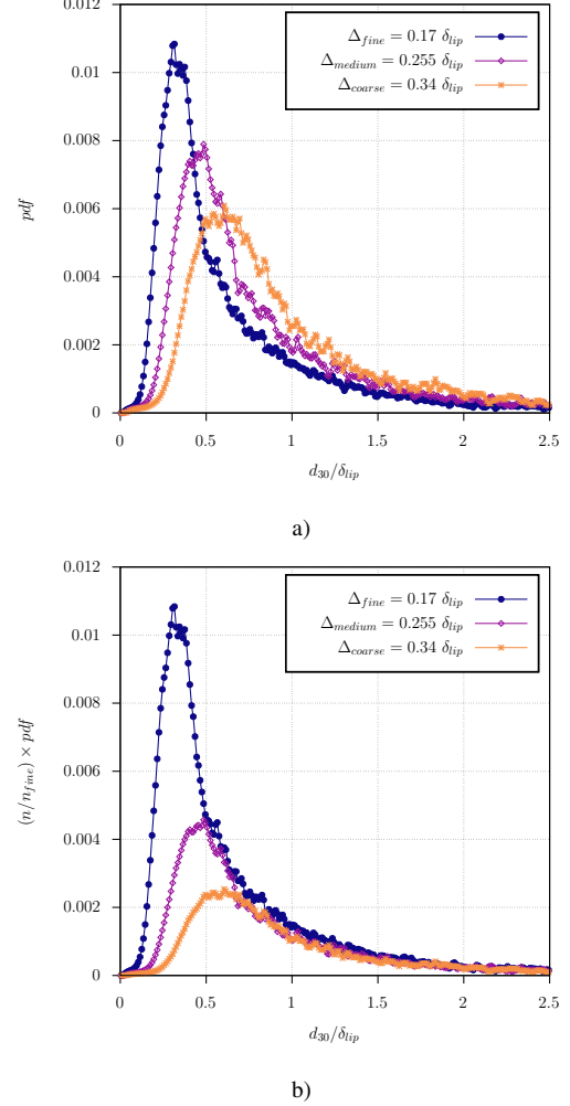
Figure 2: Probability density functions obtained on different mesh resolutions. a) pdf estimation using the formula (19), b) pdf with a scaling factor (n/n_{fine}) .
