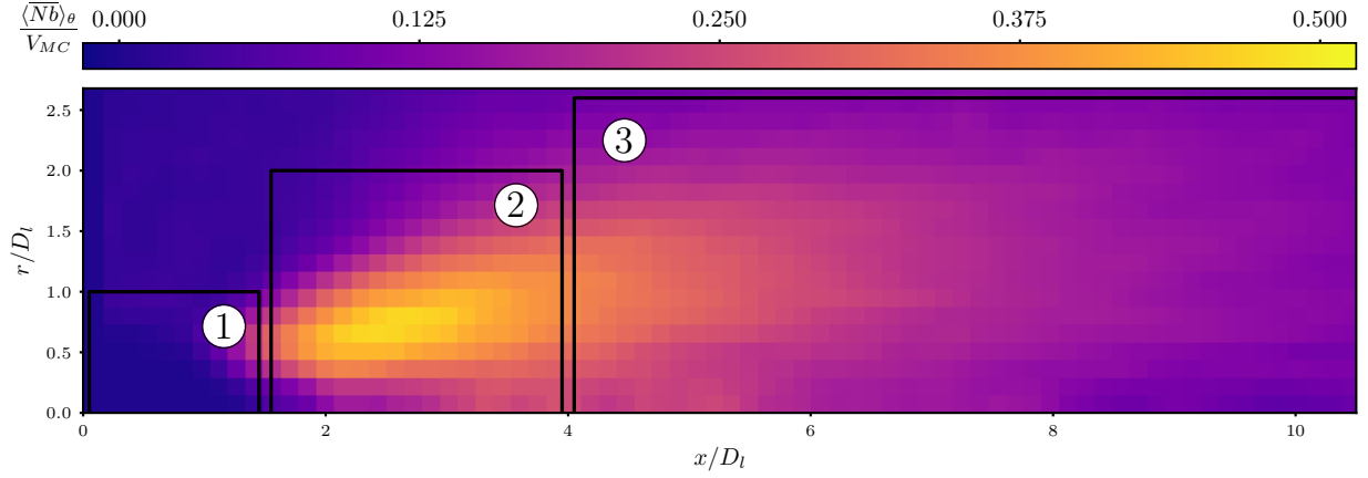
Figure 12: Density of valid detached liquid structures ( mm^{-3} ). Count gathered in all snapshots recorded in the DNS.
