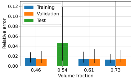
MipDMN; with material rotations
