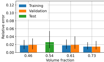
MipDMN; without material rotations
