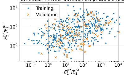
Contrasts in moduli between the phase 1 and 2
