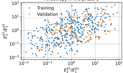
Anisotropy in the phase 1
