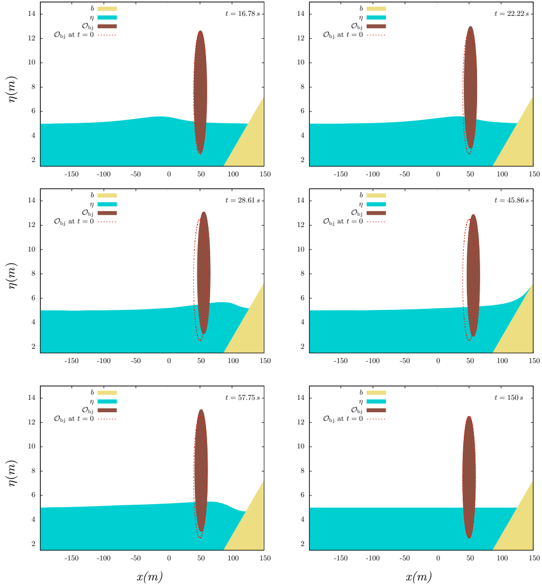
Figure 19: Test 4.6 - Nonlinear interactions with a single surface-wave: varying bathymetry and wet-dry front - Free-surface elevation for different values of time in the range [16.78 \text{ s}, 150 \text{ s}] , for n_{el}^e = 70 and n_{el}^i = 10 .
