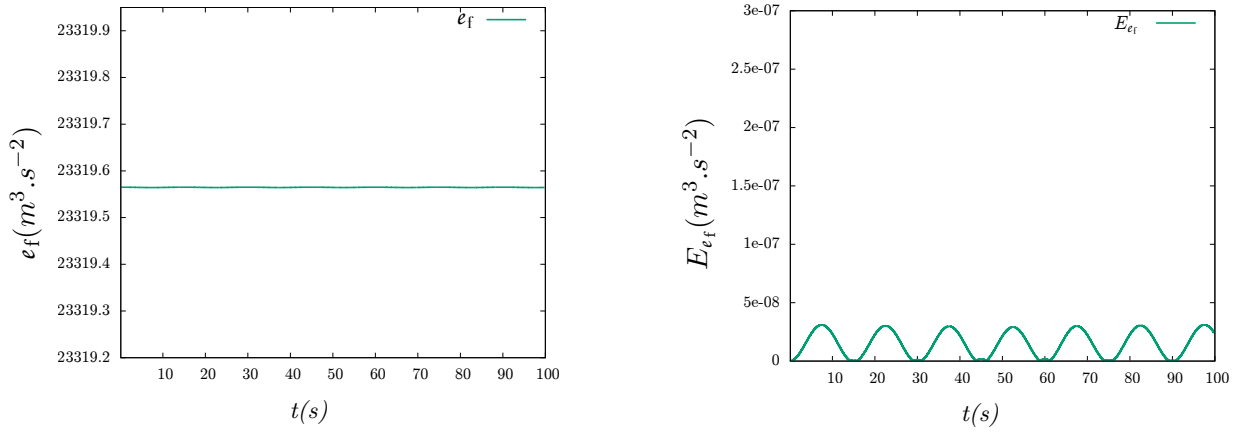
Figure 8: Test 4.2 - Elementary prescribed motions: pure heaving - Total energy and relative error, for k = 3 , n_{e1} = 200 in the range [0 \text{ s}, 100 \text{ s}] .
