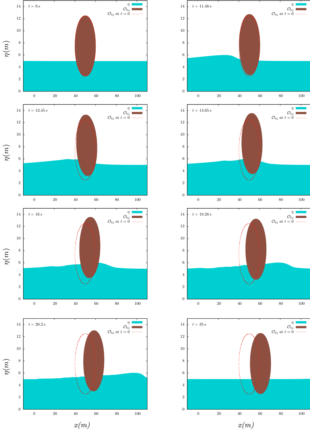
Figure 13: Test 4.4 - Nonlinear interactions with a single surface wave - Free-surface elevation computed for different values of time in the range [0\text{ s}, 35\text{ s}] for k = 3 , n_{e1}^e = 50 and n_{e1}^i = 10 .
