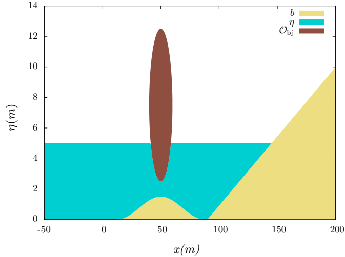
Figure 4: Test 4.1 - Preservation of a motionless steady-state - Free-surface elevation at t = 50 \text{ s} for k = 3 and n_{\text{el}}^e = 50 , n_{\text{el}}^i = 10 .
