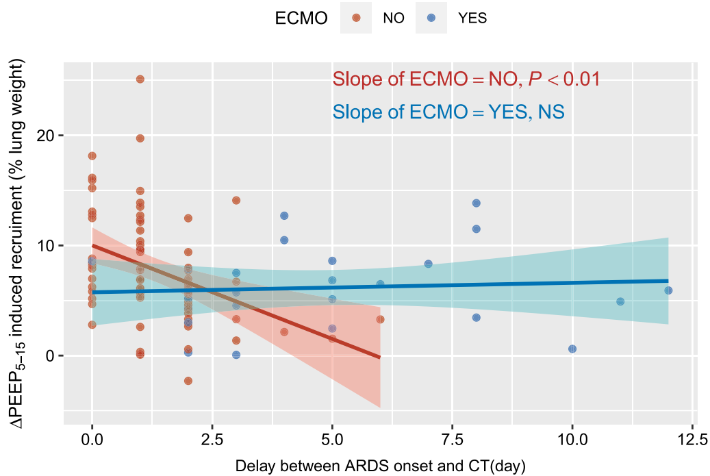
Fig. 5 Relationship between \Delta\text{PEEP}_{5-15} -induced recruitment and delay between ARDS onset and CT, according to ECMO status. Each point is partial residuals of the multivariate model with \Delta\text{PEEP}_{5-15} -induced recruitment as the dependent variable, and the following independent variables: EELV at PEEP 5 cmH 2 O, poorly inflated lung at PEEP5 and the interaction between ECMO status x delay between CT and ARDS onset. Lines are regression lines according to ECMO status. Shaded areas are 95% confidence interval for each regression line. ARDS, acute respiratory distress syndrome, CT, computed tomography, ECMO, extracorporeal membrane oxygenation, \Delta\text{PEEP}_{5-15} -induced recruitment, amount of recruitable lung between PEEP 5 and 15 cmH 2 O, EELV, end-expiratory lung volume, NS, non-statistically significant, PEEP, positive end-expiratory pressure
