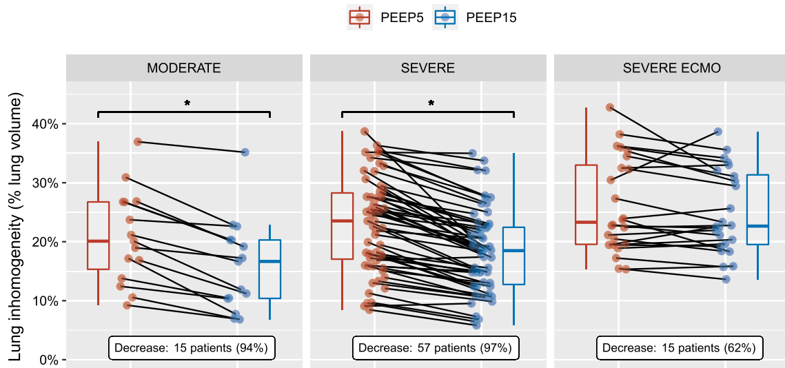
Fig. 6 Lung inhomogeneities and PEEP. The extent of lung inhomogeneity of the individual patients with moderate ARDS (left panel), severe ARDS without ECMO (middle panel), and severe ARDS with ECMO (right panel) is reported at PEEP 5 (red circles) and 15 cmH 2 O (blue circles) * p < 0.05 between PEEP 5 and 15 cmH 2 O of the same category of severity. Lung inhomogeneities are registered to the following patent: WO 2013/088336, and agreement to use this patent for research purposes was obtained from the owner (Fondazione IRCCS Ca' Granda Ospedale Maggiore Policlinico). ARDS, acute respiratory distress syndrome, ECMO, extracorporeal membrane oxygenation, MODERATE, moderate ARDS, PEEP, positive end-expiratory pressure, SEVERE, severe ARDS without ECMO, SEVERE ECMO, severe ARDS under ECMO.
