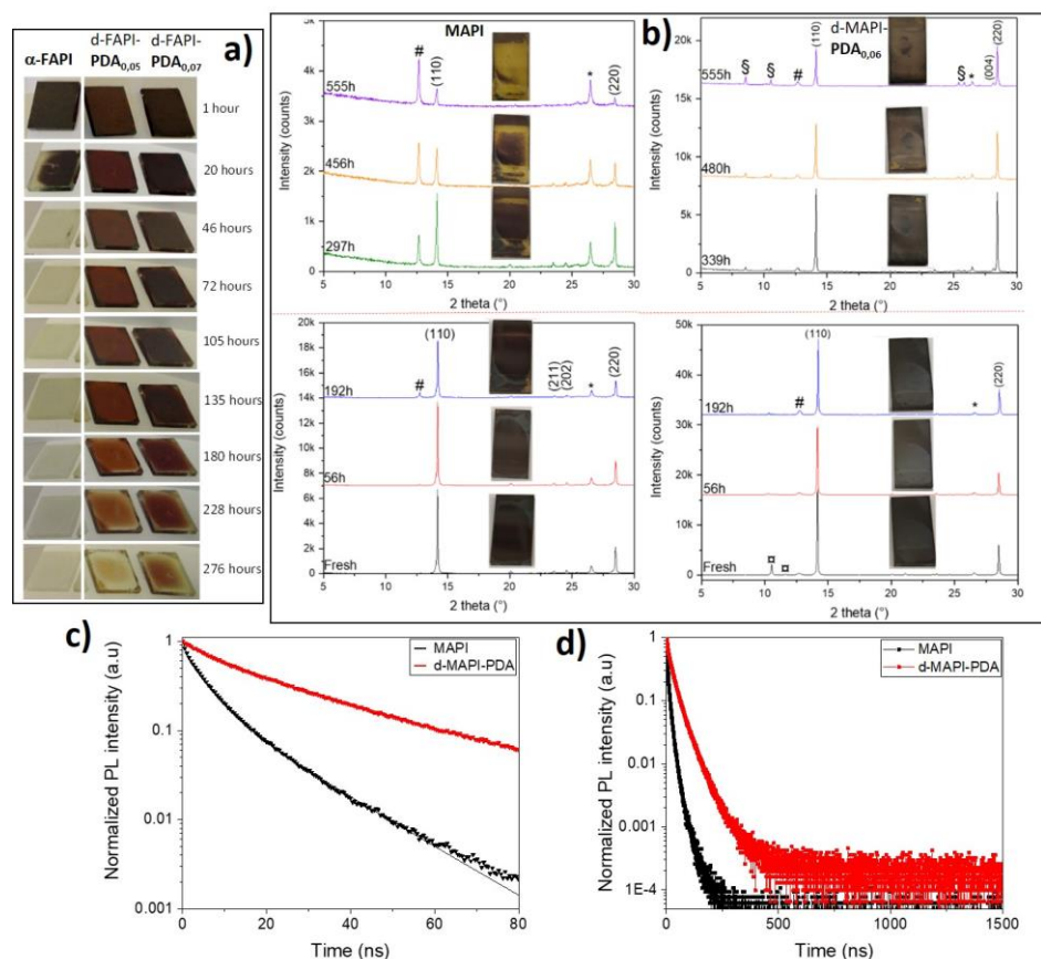
Figure 4. a) Images of thin films of \alpha -FAPbI 3 and d-FAPbI 3 -PDA x ( x = 0.05, 0.07 ) during the aging process (65–80 % RH, T = 20 – 21^\circ\text{C} ) and corresponding images of thin films of MAPI (left) and d-MAPI-PDA (right). FTO peaks are indicated by the * symbol. # indicates PbI 2 phase. \alpha indicates unknown phase present in the fresh d-MAPI-PDA film. § indicates unknown phase appearing during the aging. c) Normalized time-resolved photoluminescence of MAPI (black trace) and d-MAPI-PDA (red trace) films on FTO/c-TiO 2 substrates measured up to 80 ns. The full lines are the fit curves. d) Same as c) measured up to 1500 ns.
