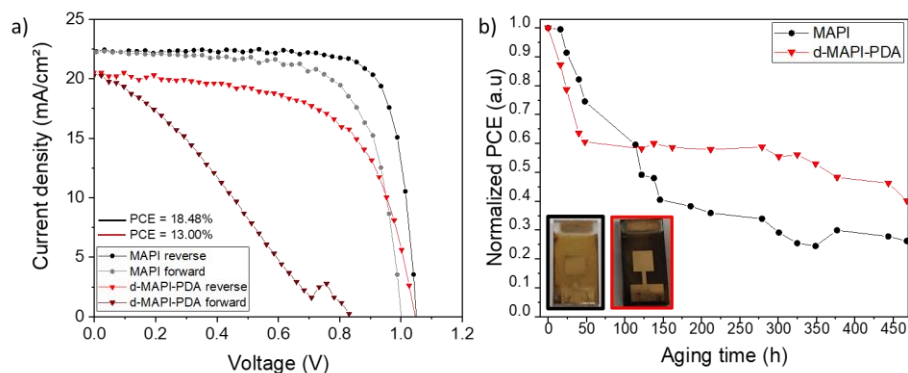
Figure 5. (a) J-V curves of best MAPI and d-MAPI-PDA devices. (b) Normalized PCE evolution of unencapsulated MAPI and d-MAPI-PDA devices efficiency as a function of aging time. Storage was made under ambient conditions (70-90 % RH, T°=16-18°C) and ambient light. Inset: Pictures of MAPI (black frame) and d-MAPI-PDA (red frame) devices after 450h of aging.
