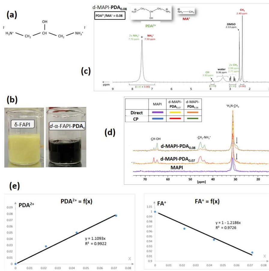
Figure 1. (a) PDA 2+ cation (with I - counterions represented) (b) Room temperature synthesis of \delta -FAPI (yellow) and d - \alpha -FAPI-PDA x (black), a lead and iodide deficient 3D halide perovskite containing PDA 2+ dication (c) 1 H NMR of d -MAPI-PDA 0.08 crystallized powder solubilized in DMSO- d 6 (d) 13 C direct excitation and cross-polarization (CP) solid state NMR of d -MAPI-PDA x crystallized powders and MAPbI 3 (e) Linear relationships of PDA 2+ and FA + contents with x ( x = number of lead and iodide vacancies), leading to the proposed formulation of (PDA) 1-11x (FA) 1-1,22x [Pb 1-x I 3-x ] for d - \alpha -FAPI-PDA compounds.
