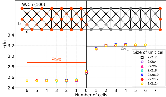
Figure 2: Inter-layer distance c in the Z direction of the W/Cu super-cell. The black line displays the interface. We numbered the layers starting from the interface. Above the graph, we schematically represent the (100) crystallographic plane of the (2 \times 2 \times 14) W/Cu: the orange and gray points are the positions of Cu and W atoms, respectively. The light-orange and light-gray points represent the positions of Cu and W atoms in the (200) plane, respectively. The horizontal orange and gray lines the c parameter of \text{Cu}^{\text{bcc}} and \text{W}^{\text{bcc}} respectively: c_{\text{Cu}^{\text{bcc}}} = 2.871 \text{ \AA} and c_{\text{W}^{\text{bcc}}} = 3.187 \text{ \AA} .
