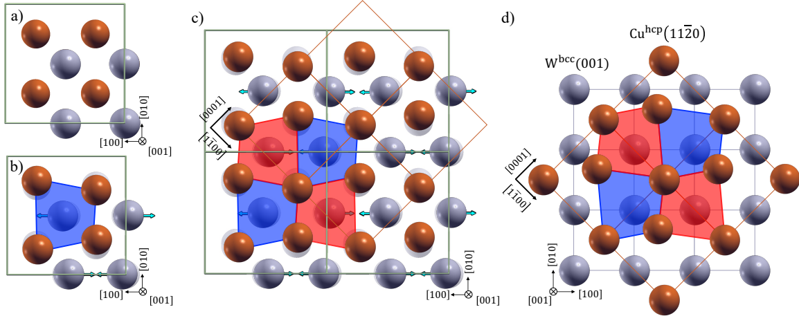
Figure 3: Reconstruction of the Cu network. a) Before geometry relaxation, b) after geometry relaxation, c) same as b) but at a larger scale, and d) the \text{Cu}^{\text{hcp}}(11\bar{2}0) on \text{W}^{\text{bcc}}(001) experimentally observed by Wormeester et al. [6] and Bollmann et al. [8]. The blue and red surfaces represent the regions with similar deformations.
