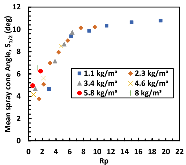
Figure 7. Evolution of the mean spray angle for the half-penetration versus the superheat degree.
