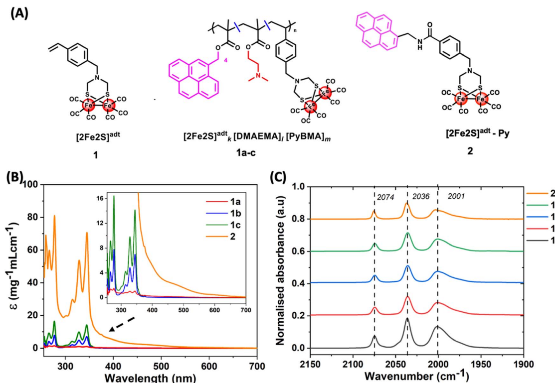
Fig. 1 (A) Schematic representation of synthesized compounds, i.e. , complex 1 (synthetic precursor of the metallopolymers), metallopolymers 1a–c and complex 2 , (B) UV-vis spectra of 1a–c (197; 50 and 20 \mu\text{g mL}^{-1} ) and 2 (11 \mu\text{g mL}^{-1} ) in DMF (C) Infrared spectroscopy of 1 , 1a–c and 2 in \text{CHCl}_3 using transmission mode. The intensity of FTIR traces of 1a were multiplied by 3 and 1b and 1c multiplied by 10 each to have between comparison with 1 and 2 . Here k : l : m is the ratio of [\text{2Fe}_2\text{S}]^{\text{adt}} : [\text{DMAEMA}]_l : [\text{PyBMA}]_m . The exact details of the ratio for each metallopolymers were mentioned in Table 1.
