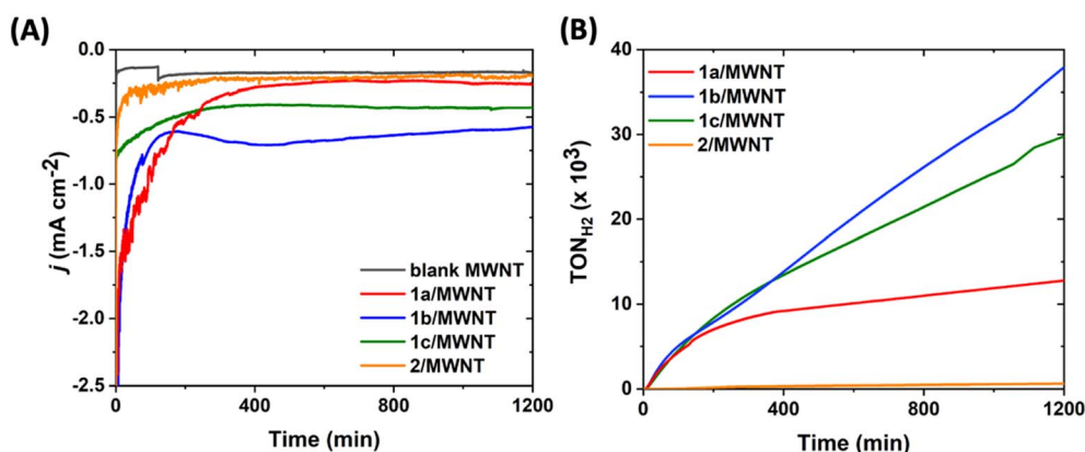
Fig. 3 CA of metallopolymers 1a–c and complex 2 immobilized on MWNT/GCE. (A) Current density ( j ) vs. time; (B) turnover number ( \text{TON}_{\text{H}_2} ) vs. time recorded during CA at -0.49 \text{ V vs. RHE} in 0.2 \text{ M} sodium phosphate buffer, pH 7 under continuous flow of \text{N}_2 ( 5 \text{ mL min}^{-1} ). Here, bare MWNT, 1a /MWNT, 1b /MWNT, 1c /MWNT and 2 /MWNT are represented by grey, red, blue, green and orange colors, respectively. The \text{TON}_{\text{H}_2} were calculated using loading from ICP-OES assessment.
