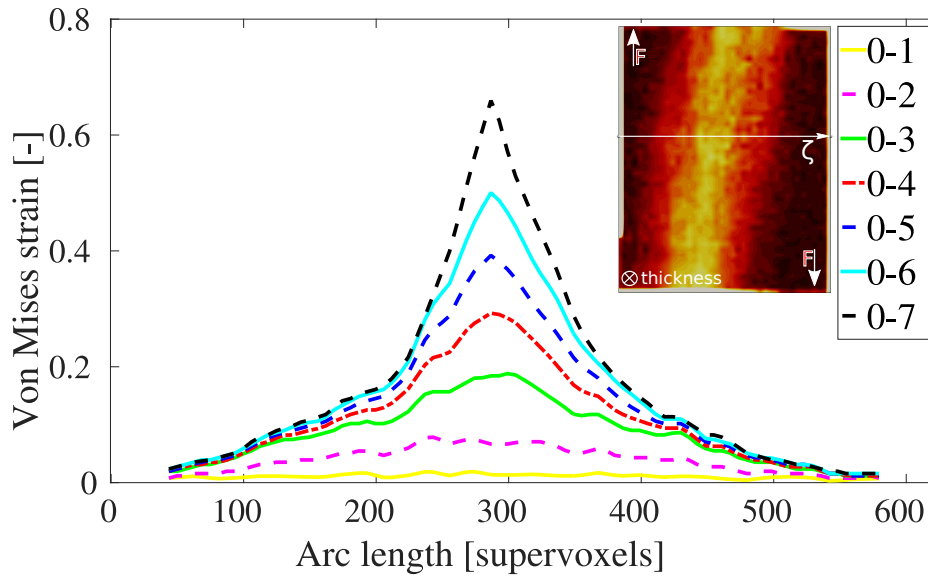
Figure 9: Von Mises strain profiles from cumulated incremental DVC calculations. The position of the profile axis \zeta is denoted on the strain map illustration
