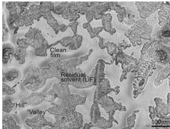
Figure 8. Confocal laser microscopy image of the top surface of as-grown Er:LiYF 4 thin film. Microscope objective 20×, bright field, reflection mode, \lambda = 405 nm.
