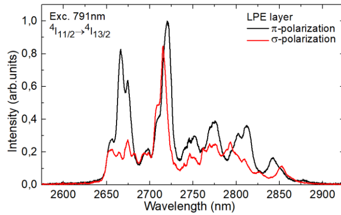
Figure 15. Polarized mid-infrared luminescence spectra of Er 3+ ions from the Er:LiYF 4 epitaxial layer, \lambda_{\text{exc}} = 791 nm. The light polarizations are \pi and \sigma .
