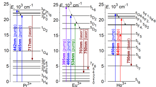
Fig. 1. Energy-level schemes of Pr 3+ , Eu 3+ and Ho 3+ ions showing pump and deep-red laser transitions.
