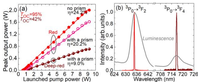
Fig. 5. Diode-pumped deep-red / red Pr fiber lasers: (a) input-output dependences, \eta – slope efficiency; (b) typical spectra of laser emission, grey curve – luminescence spectrum.
