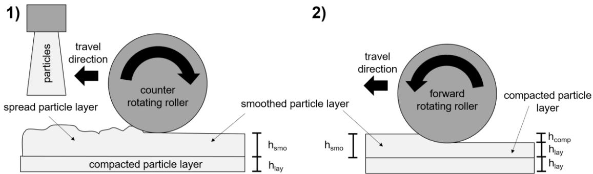
Figure 4: Schematic illustration of particle spreading and smoothing (1) and compaction (2)
