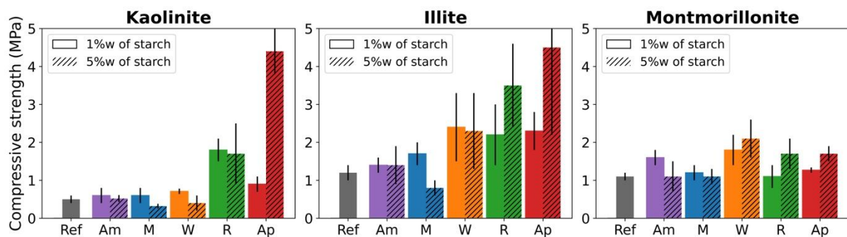
Figure 3 : Compressive strength of mortar mixes. From left to right: kaolinite, illite, and montmorillonite results. In grey: reference (Ref); purple: starch from maize with high amylose content (Am); blue: starch from maize (M); orange: starch from wheat (W); green: starch from rice (R); red: amylopectin (Ap)
