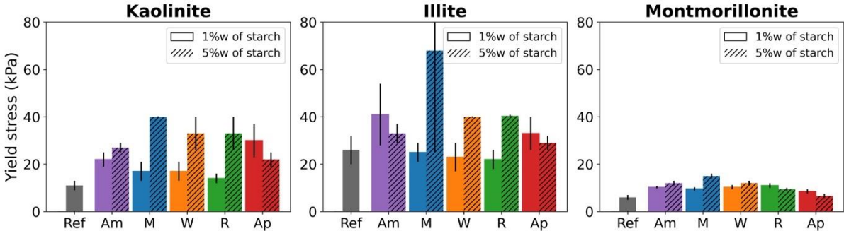
Figure 5 : Yield stress of mortar mixes. From left to right: kaolinite, illite, and montmorillonite results. In grey: reference (Ref); purple: starch from maize with high amylose content (Am); blue: starch from maize (M); orange: starch from wheat (W); green: starch from rice (R); red: amylopectin (Ap)
