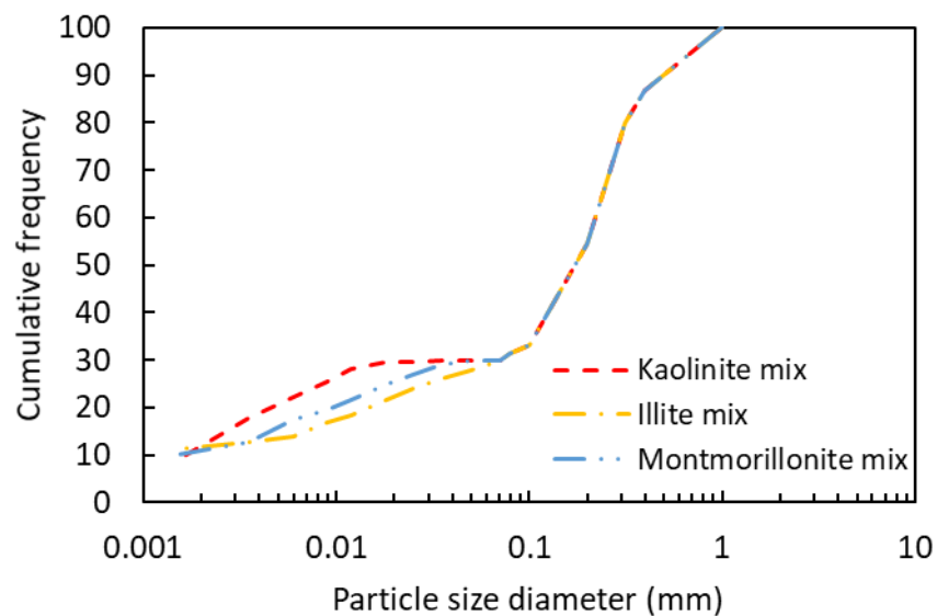
Figure 2 : Particle size distribution of reference mixes
