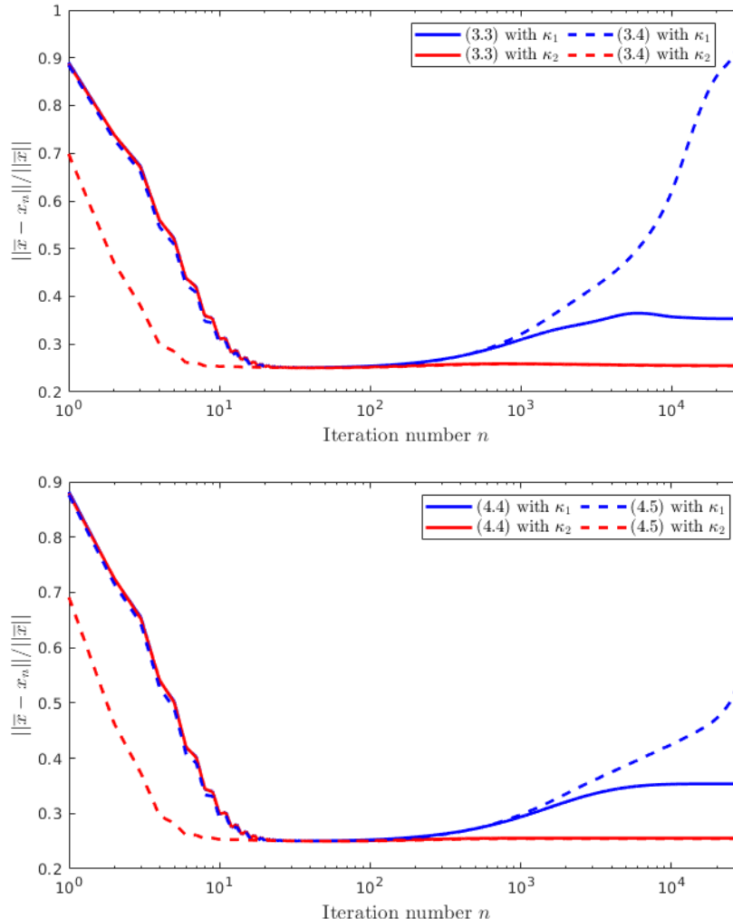
Fig. 2: Evolution of the error (\|\bar{x} - x_n\|/\|\bar{x}\|)_n along iterations for Algorithms (III.3)-(III.4) (top) and Algorithms (IV.4)-(IV.5) (bottom), for two settings of parameter \kappa .
