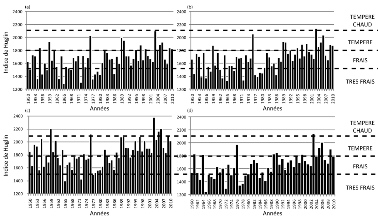
Figure 42: Evolution of the Hugin Index for 4 weather stations (a: Nantes, b: Angers, c: Saumur, d: Tours) in the Loire Valley during the period 1950/60 to 2010 (Bonnefoy et al. 2012)
