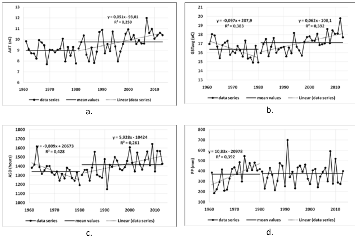
Figure 22: Climate change indicators in Cotnari (Weather Station of Cotnari, INMH Romania): a. average annual temperature (AAT); b. growing season temperature (GSTavg); c. actual sunshine duration (ASD); d. precipitation during the growing season (PP). All displayed R^2 and regression coefficients' values are significant for p=0.05 .
