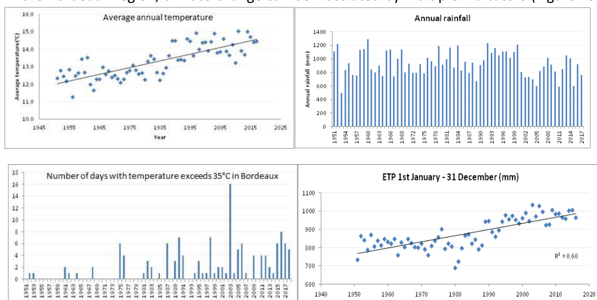
Figure 29: Climate change indicators in Bordeaux (Météo France weather station of Mérignac).
