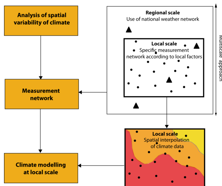
Figure 2. Local-scale climate modelling approach, based on measurements from a climate sensors network established to reflect local factors
