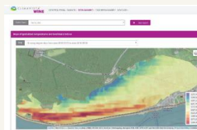
MAP OF THE GROWING DEGREE DAYS INDEX IN 2016 OVER RHEINGAU PILOT SITE
