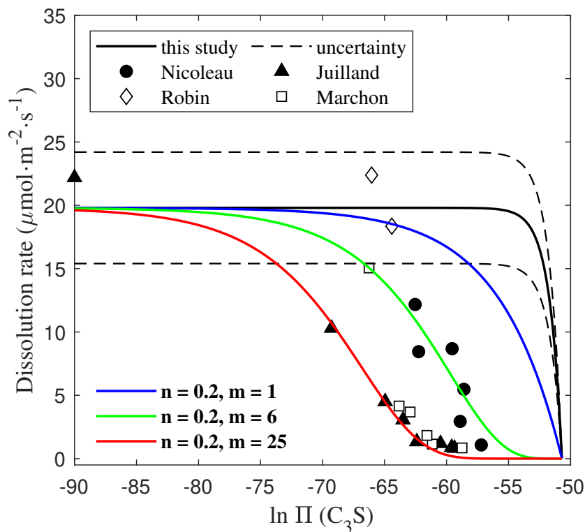
Figure 9: Dissolution rate of C_3S as a function of the natural logarithm of the ionic activity product of the solution ( \text{Ca}_3\text{SiO}_5 + 5\text{H}_2\text{O} \rightarrow 3\text{Ca}^{2+} + \text{H}_4\text{SiO}_4 + 6\text{OH}^- ). The black solid line represents the dissolution of C_3S in deionized water and is a non-sigmoidal function complying with TST (black dashed lines below and above display the experimental uncertainty due to the standard deviation on the rate constant k_{C_3S} ). Blue circles: data from Nicoleau et al. [18] and collected in a reactor connected to an ICP spectrometer. The data with the same [\text{CaO}]_{aq} into the initial solution (5, 5.5, 8.5, 10.5, 11 and 15 mM) and w/s = 10 were averaged. Black triangles: data from Juilland and Gallucci [13] collected with the aid of a flow-through-cell and VSI measurements. White diamonds: data from Robin et al. [20]. White squares: data from Marchon et al. [21]. Functions including n and m parameters were added in different colors.
