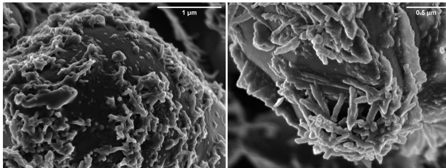
Figure 3: SEM micrograph of the surface of the hydrated platelet of \text{C}_3\text{S} at 45 min (left) and 120 min (right). The C–S–H needles are distributed on the surface of the hydrated sample. SEM micrographs were collected on dried surfaces coated with a layer of graphite. The secondary electron images were acquired with a TESCAN Solaris FEG-SEM at low voltage (2 KeV) to avoid surface charging and high vacuum mode.
