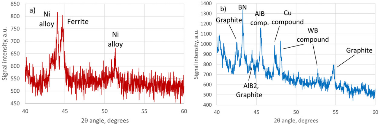
Figure 2: XRD spectra of the magnetic (a) and non-magnetic (b) dust batches from AUG. It should be noted that the W peaks are located outside the depicted spectral window in order to increase the readability of the most significant spectral range.
