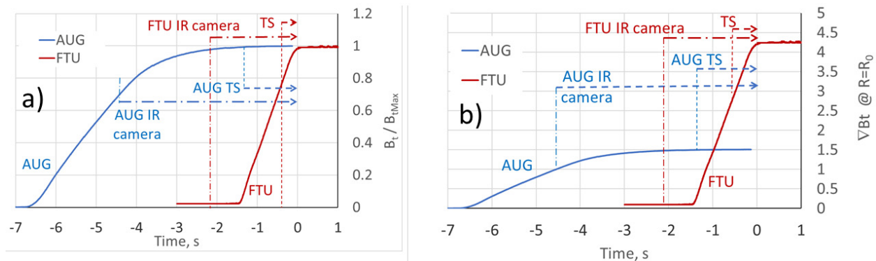
Figure 3: Temporal evolution of a) B_t/B_{tMax} , b) \nabla_{B_t} for typical AUG (#40373) and FTU (#40819) discharges with B_{tMax}(AUG) = -2.5 T and B_{tMax}(FTU) = 4 T. Note that \nabla_{B_t} is evaluated at the low position R = R_0 for both devices; R_0(AUG) = 1.65 m and R_0(FTU) = 0.935 m.
