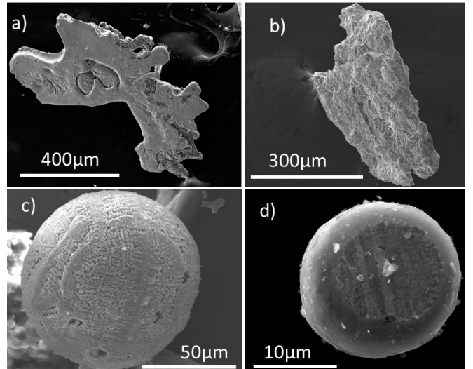
Figure 1: SEM images of magnetic dust collected from AUG. a) Ni-based splash (back view), b) flake (steel), c) near-spherical dust (steel) with dendrite textured surface, d) near-spherical dust (steel) without dendrite texture.
