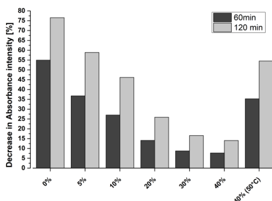
Figure 5: Variation of UV absorption at maximum absorption of sensor 5 ( 1 \cdot 10^{-5}\text{M} , 25°C or 50°C) upon addition of 100 equivalents of hydrazine in acetonitrile containing increasing water content.
