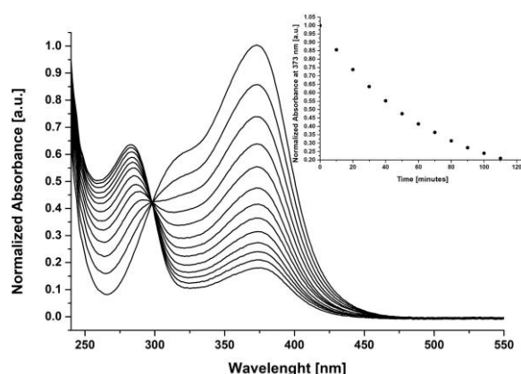
Figure 2: UV absorption of sensor 5 ( 1 \cdot 10^{-5} \text{M} , 25^\circ \text{C} ) upon addition of 100 equivalents of hydrazine in acetonitrile. Spectra acquired every 10 min. Inset: variation of absorbance at 373 nm
