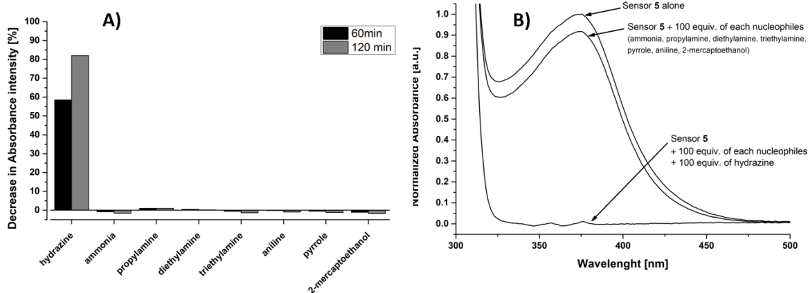
Figure 3: A) Variation of UV absorption at 373 nm of sensor 5 ( 1 \cdot 10^{-5} \text{M} , 25^\circ \text{C} ) upon addition of 100 equivalents of different competing nucleophiles in pure acetonitrile. B) UV spectra of sensor 5 alone, then 2h after addition of 100 equivalents of each competing nucleophiles and finally 2h after addition of 100 equivalent of hydrazine.
