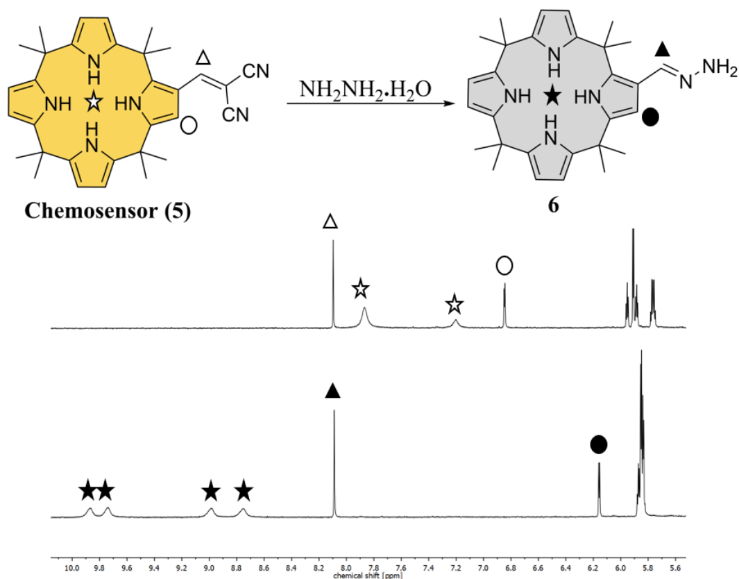
Figure 1 : Partial ^1\text{H} NMR spectra (400 MHz, \text{CD}_3\text{CN} , 298K) of sensor 5 before (top) and after (bottom) addition of an excess of hydrazine. (full spectra are provided in Figure S5)
