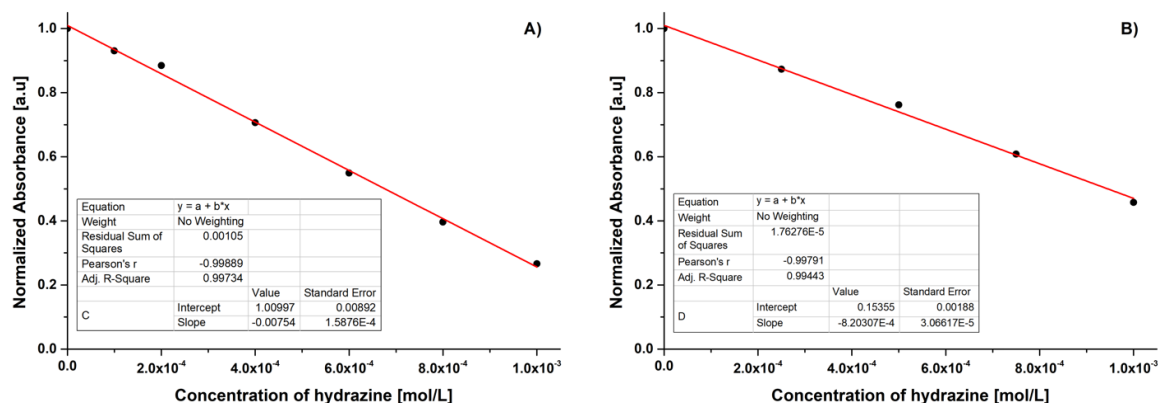
Figure 6 : Calibration curves for hydrazine monitoring in the range 10-1000 \mu\text{M} obtained after 2h of incubation. A) in acetonitrile, 25 ^{\circ}\text{C} B) ACN-Water 40%, 50 ^{\circ}\text{C}
