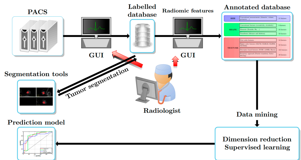
Figure 1. Radiomics pipeline.
