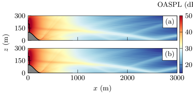
FIG. 12. OASPL at \beta = 0^\circ for the hill case computed using (a) LEE and (b) \text{WAPE}_{\text{topo}} .
