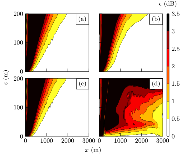
FIG. 7. \Delta L difference computed between the LEE and (a,b) \text{WAPE}_{\text{vec}} and (c,d) \text{WAPE}_{\text{topo}} for (a,c) an atmosphere at rest and (b,d) for an ABL profile with 10 \text{ m s}^{-1} at hub height. The results are averaged over N_f = 35 frequencies, see Table I, and are computed for flat terrain.
