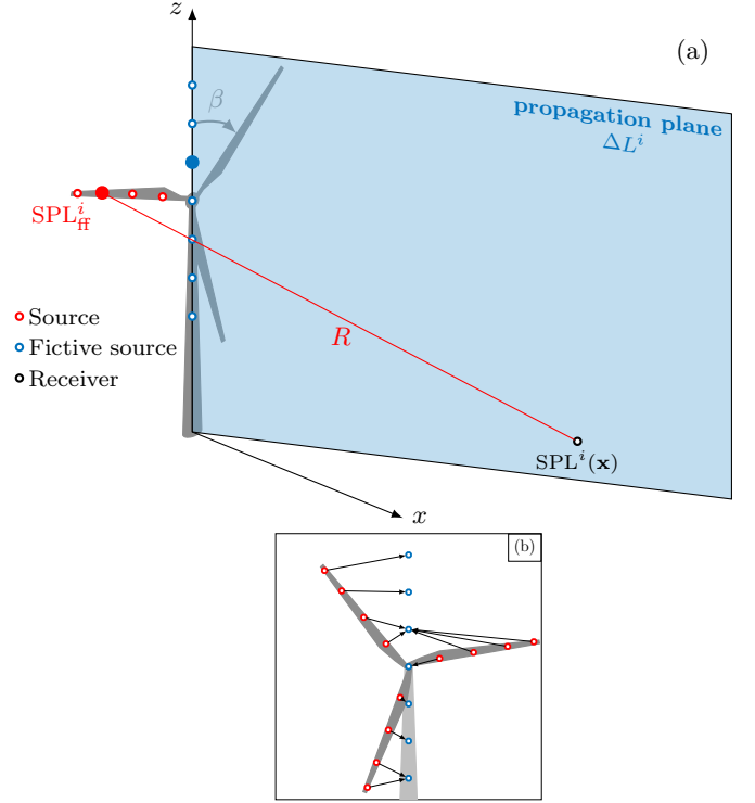
FIG. 2. (a) Calculation of the SPL at a receiver due to one blade segment. (b) Total SPL from all segments is determined using the closest fictive source to compute the \Delta L .
