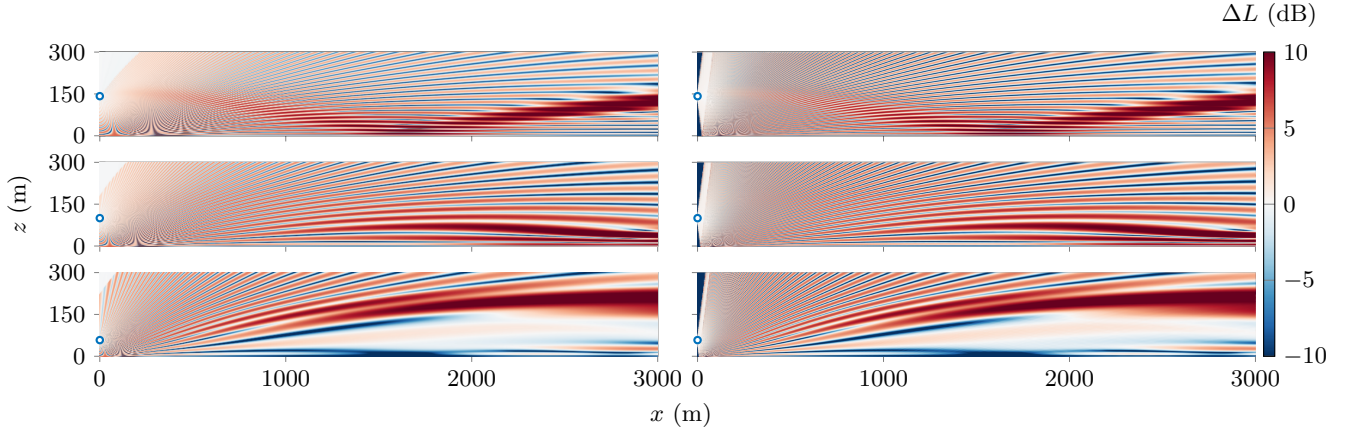
FIG. 5. \Delta L computed with LEE (left) and \text{WAPE}_{\text{vec}} (right) at 100 Hz for several source heights (circles): 142 m (top), 100 m (middle), and 58 m (bottom).
