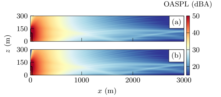
FIG. 8. OASPL at \beta = 0^\circ for the flat case computed using (a) LEE and (b) \text{WAPE}_{\text{topo}} .
