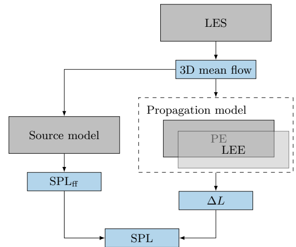
FIG. 1. Diagram of the complete prediction methodology
