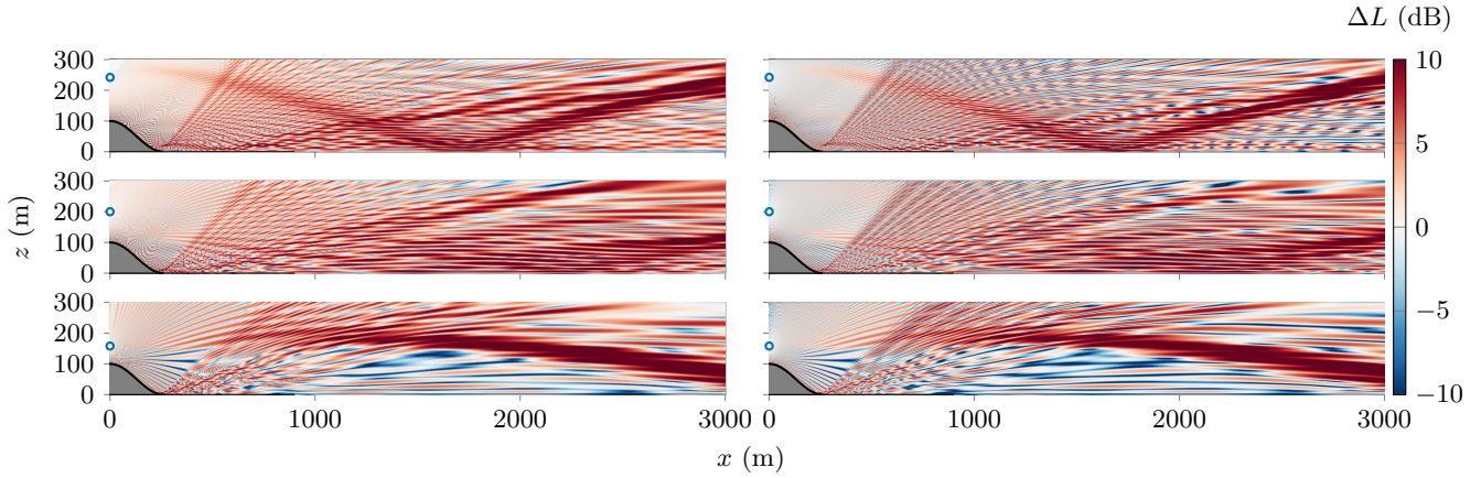
FIG. 10. \Delta L computed with LEE (left) and \text{WAPE}_{\text{topo}} (right) at 100 Hz for several source heights (circles): 242 m (top), 200 m (middle), and 158 m (bottom).
