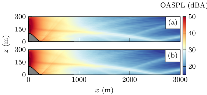
FIG. 12. OASPL at \beta = 0^\circ for the hill case computed using (a) LEE and (b) WAPE_{topo} .
