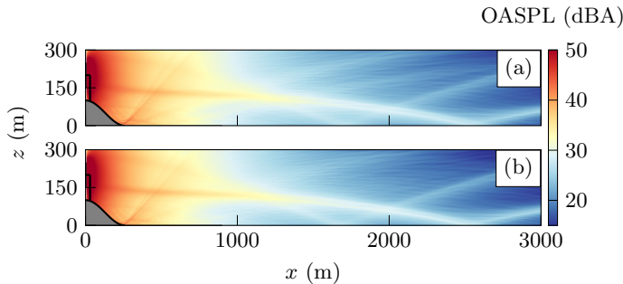
FIG. 12. OASPL at \beta = 0^\circ for the hill case computed using (a) LEE and (b) \text{WAPE}_{\text{topo}} .
