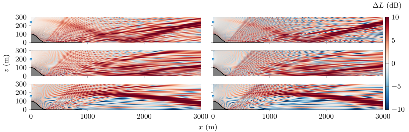
FIG. 10. \Delta L computed with LEE (left) and WAPE_{\text{topo}} (right) at 100 Hz for several source heights (circles): 242 m (top), 200 m (middle), and 158 m (bottom).
