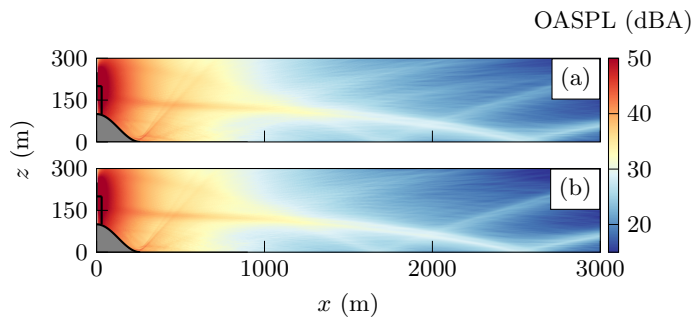
FIG. 12. OASPL at \beta = 0^\circ for the hill case computed using (a) LEE and (b) WAPE_{\text{topo}} .
