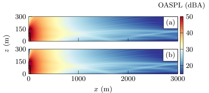
FIG. 8. OASPL at \beta = 0^\circ for the flat case computed using (a) LEE and (b) \text{WAVE}_{\text{topo}} .
