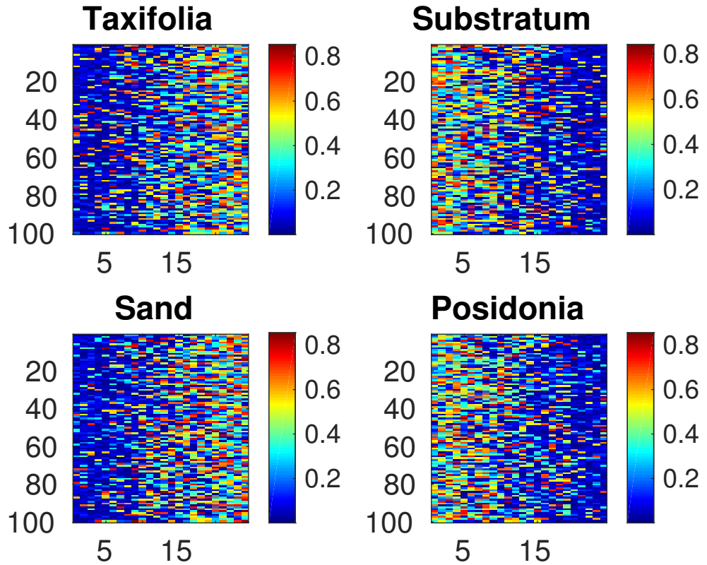
Figure 2. Maps of coefficients a_{j,i} for all classes of pure materials (Caulerpa Taxifolia, substratum, sand and Posidonia). We numerically generated the coefficients a_{j,i} and p_{n,i} of (6), so as to simulate relevant pure material “abundances”. To this end, we used the same protocol as in [50]. The considered images contain 100 \times 24 pixels.
