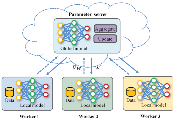
FIG. 3. Distributed learning [17].
