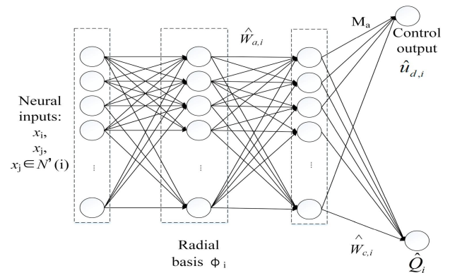
FIG. 4. Integrated actor-critic network [19].
