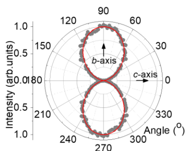
Fig. 6. Analysis of polarization state of laser emission from the deep-red Eu:CsGd(MoO 4 ) 2 laser, T_{\text{OC}} = 0.25\% , P_{\text{abs}} = 0.58 \text{ W} .
