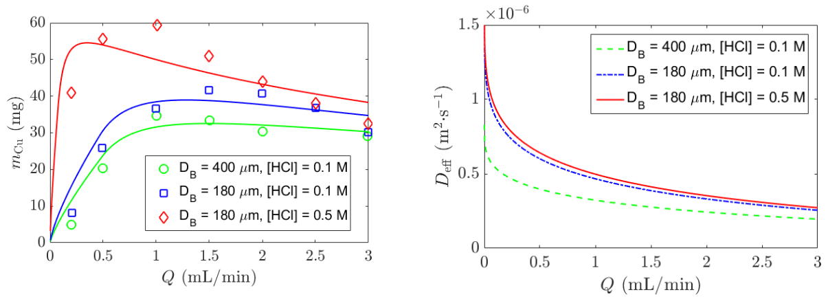
Figure 6. a) Comparison of the mass of dissolved copper measured experimentally and predicted Equation (15). b) values of D_{\text{eff}} obtained from Eq. (10) using values of \kappa that enable to fit Eq. (15) with the experimental data.
