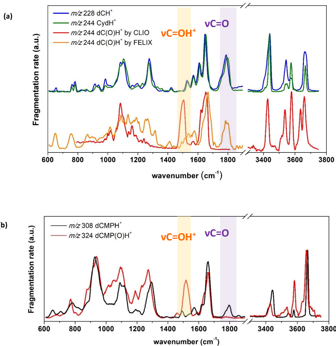
Figure 5. Comparison of the IRMPD spectra for (a) dCH + (blue), CydH + (green) and single oxidation product dC(O)H + (red recorded at CLIO, orange recorded at FELIX); (b) dCMPH + (black) and its single oxidation product dCMP(O)H + (red).
