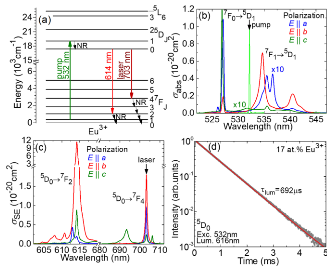
Fig. 2. (a) The energy-level diagram of \text{Eu}^{3+} ions; (b-d) Spectroscopy of \text{Eu}^{3+} ions in the 17 at.% \text{Eu}:\text{CsGd}(\text{MoO}_4)_2 crystal: (b) absorption cross-sections, \sigma_{\text{abs}} , the {}^7\text{F}_{0,1} \rightarrow {}^5\text{D}_1 transition; (c) SE cross-sections, \sigma_{\text{SE}} , the {}^5\text{D}_0 \rightarrow {}^7\text{F}_2 and {}^7\text{F}_4 transitions; (d) luminescence decay curve. Arrows in (b,d) indicate the pump and laser wavelengths.
