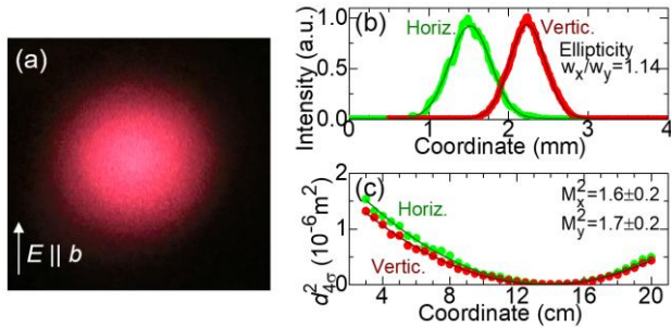
Fig. 5. Spatial characteristics of deep-red emission ( \sim 703 nm) from the Eu:CsGd(MoO 4 ) 2 laser: (a) a photograph of a laser beam on a black screen in the far-field; (b) 1D intensity profiles ( symbols – experimental data, curves – Gaussian fits); (c) evaluation of M^2_{xy} parameters.
