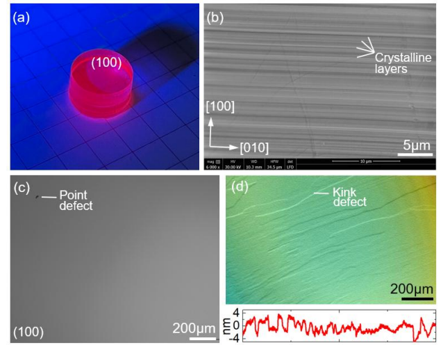
Fig. 1. Cleaving \text{Eu}:\text{CsGd}(\text{MoO}_4)_2 crystal: (a) a (100) crystal plate under illumination by a UV lamp (365 nm); (b) a FESEM image of the lateral boule side showing stacked crystalline layers; (c) a (100) cleaved crystal plane observed with a confocal laser microscope; (d) a topography map of this surface and a roughness plot across its diagonal.
