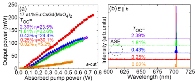
Fig. 4. Deep-red Eu:CsGd(MoO 4 ) 2 laser based on a cleaved crystal plate ( a -cut): (a) input-output dependences, \eta – slope efficiency; (b) typical spectra of laser emission, laser polarization: E \parallel b .
