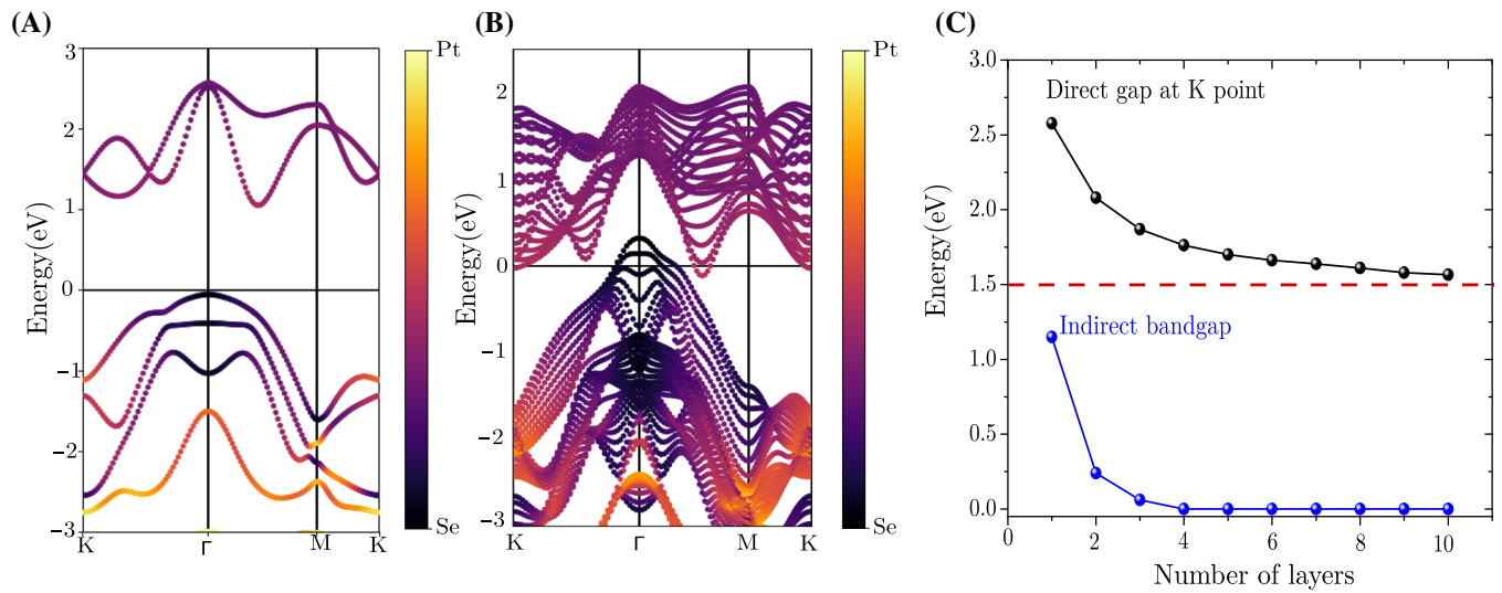
FIGURE 4 Layer dependent bandstructure of PtSe 2 . PtSe 2 band structure including spin-orbit coupling for (A) ML and (B) multilayer cases (10 ML). Energies are referenced to the Fermi level. (C) Indirect bandgap at \Gamma -M and direct bandgap at K points as a function of number of PtSe 2 layers.
