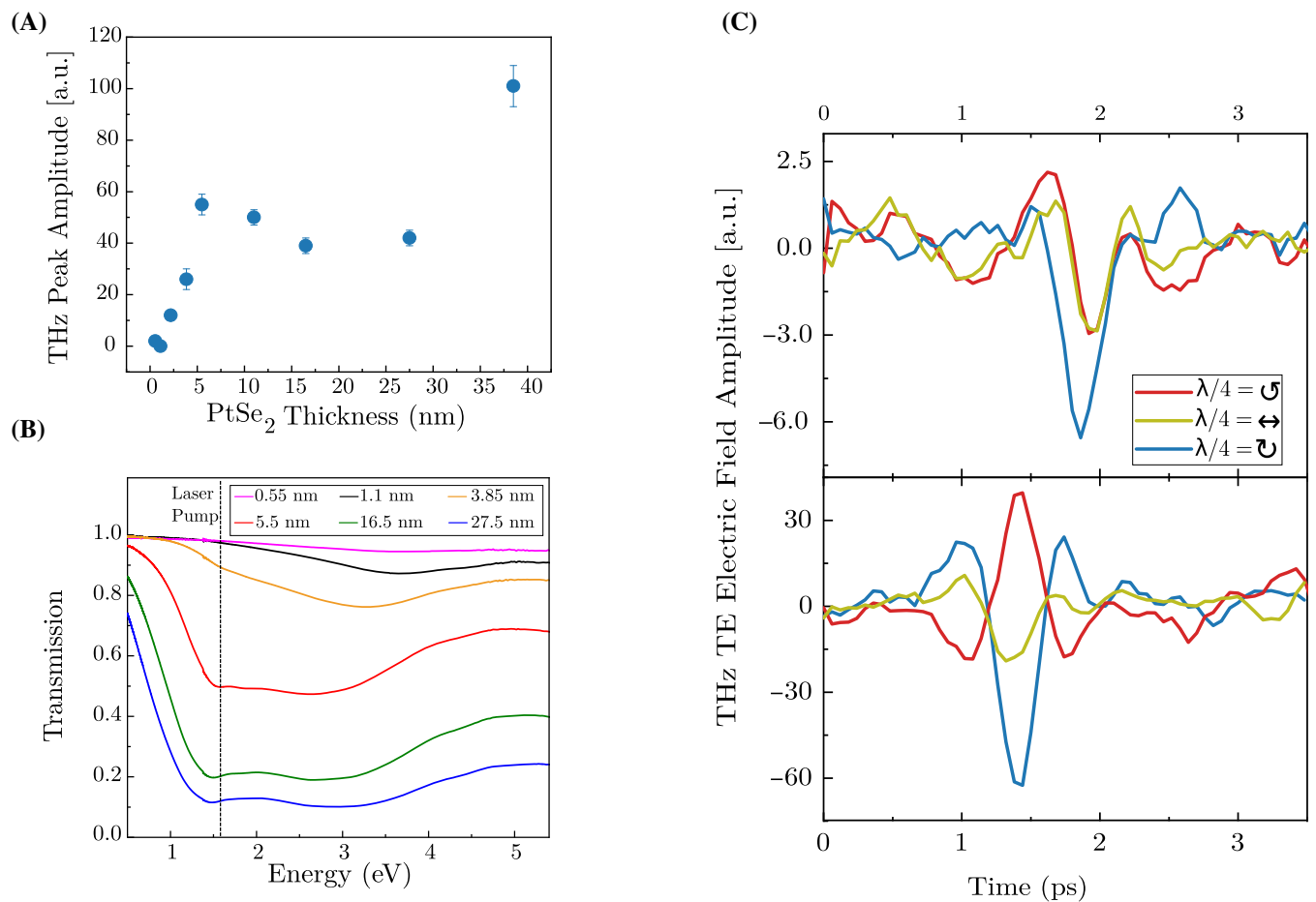
FIGURE 5 Layer controlled THz and optical properties of PtSe 2 —From monolayer to bulk. (A) THz peak amplitude as function of thickness of the PtSe 2 samples. The measurements were done in reflection geometry at 45° with TM polarization of the optical pump and THz TM generated pulse. (B) Optical transmission for different PtSe 2 thicknesses extracted over the UV, visible and near infrared spectral regions. (C) THz TE electric field of 5.5 nm (top) and 38.5 nm PtSe 2 (down) under linear (TM), LCP and RCP polarization laser excitation.
