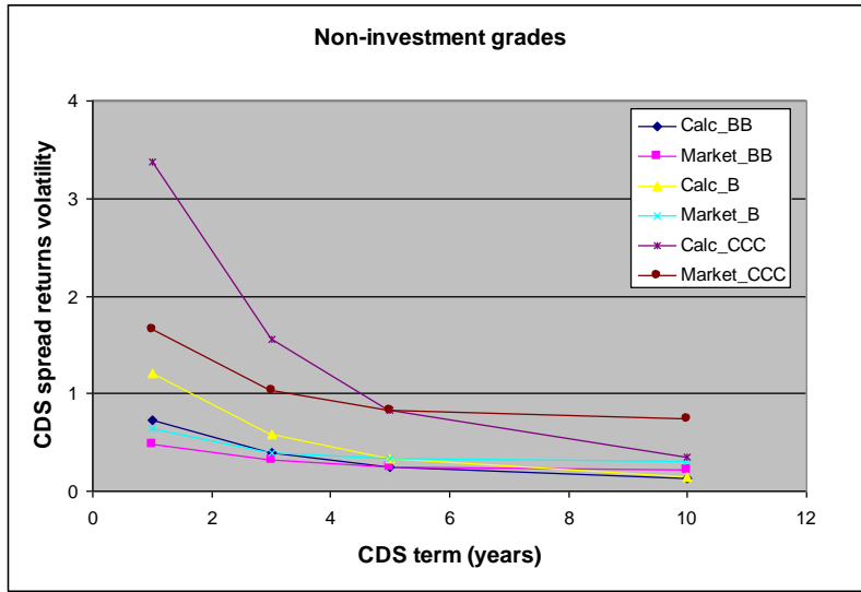
Figure 2. The calculated and market data results for non-investment grades of the global CDS indices.
