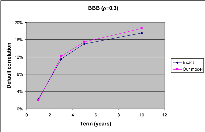
Figure 6. The calculated and exact default correlation for investment grade BBB: asset correlation is 30%
