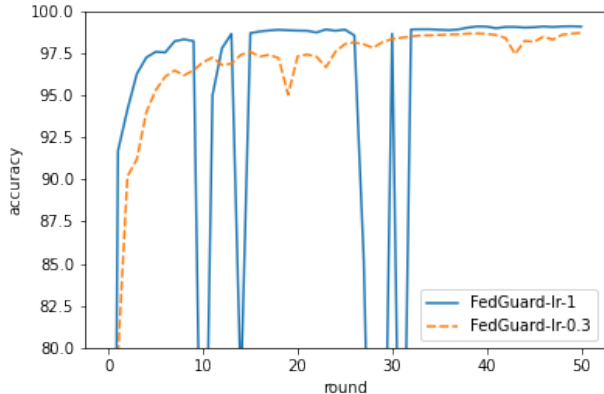
Fig. 5: Impact of learning rate on FEDGUARD stability (40% malicious peers, label flipping attack)
