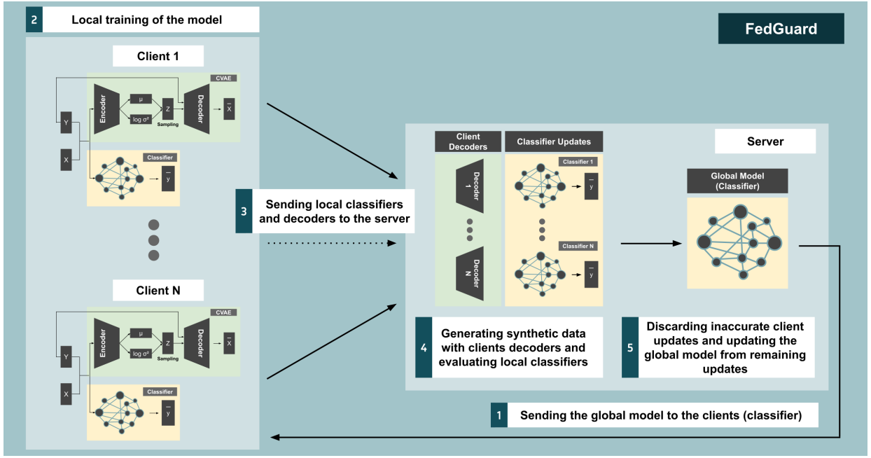
Fig. 3: FEDGUARD execution
