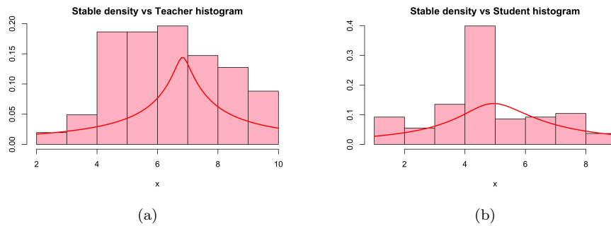
Figure 12. Stable density Estimation.
