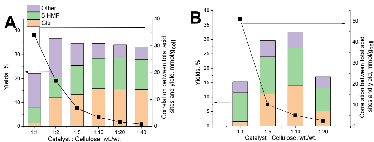
Figure 3. Correlation between the yield of products and the weight ratio of catalyst/cellulose. (A) NbZr-W3, (B) NbZr-MAW3. (Experimental conditions: 10 g L -1 of cellulose in 45 mL of reaction mixture, 1 mPa of Ar, 453 K, 7 h).
