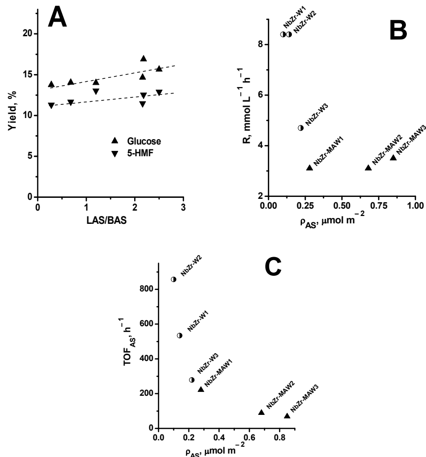
Figure 4. (A) Correlation between the yields of glucose and 5-HMF and the LAS/BAS ratio. (B) Correlation between the initial reaction rate and the density of acid sites. (C) Correlation between the TOF_{AS} and the density of acid sites.
