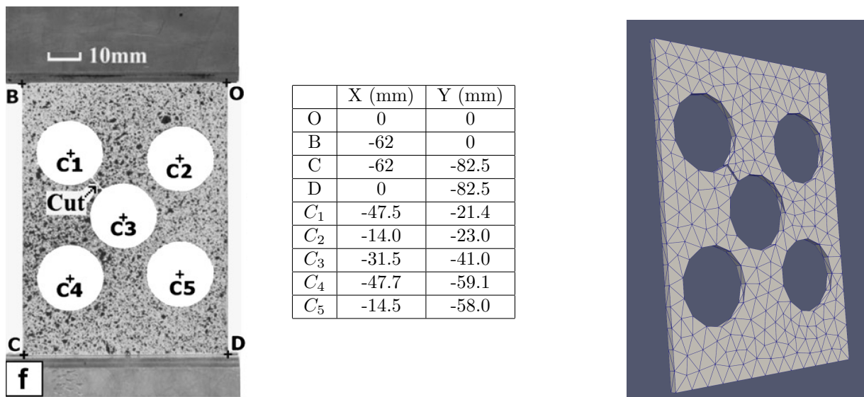
Figure 1: Geometry of the silicone sample, position of the holes and initial mesh.
