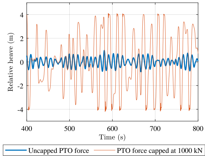
Figure 5: WEC's response in relative heave to PTO force capping
