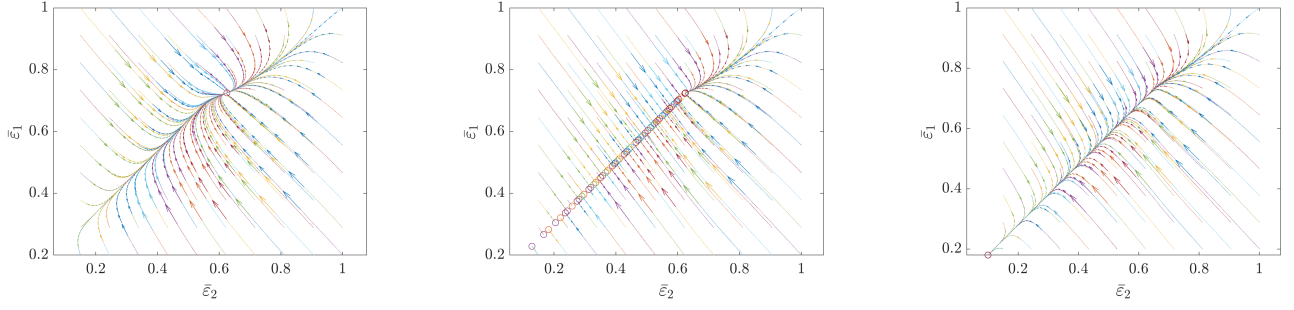
(a) \eta < \eta_c (sustainable demand regime): trajectories converge towards a unique equilibrium, \bar{\varepsilon}_D^* . (b) \eta > \eta_c (unsustainable demand regime): trajectories converge towards an infinite number of possible equilibria. (c) \eta = \eta_c (critical demand regime): trajectories converge towards an almost-empty state of charge.
