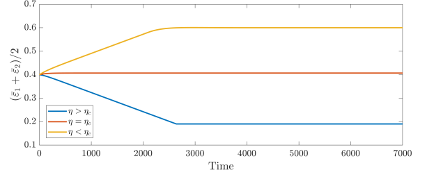
Fig. 3: Example 1. Evolution of the mean SoC of the system using the average model, for different \eta . The case \eta > \eta_c reaches a plateau representing the fact that the cars are stuck when the SoC comes near the loss of the path.
