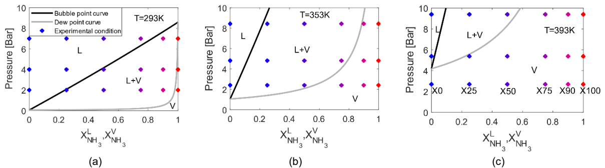
Figure 3. Vapor-Liquid Equilibrium calculation of ammonia/ethanol and experimental conditions for the three temperatures (a) 20°C (b) 80°C and (c) 120°C with the color range as a function of ammonia ratio
