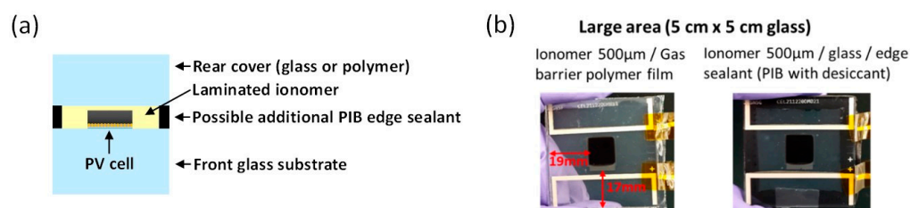
Figure 2. (a) Architecture of the encapsulated PV devices; (b) photographs of the 2 encapsulation combinations here selected.
