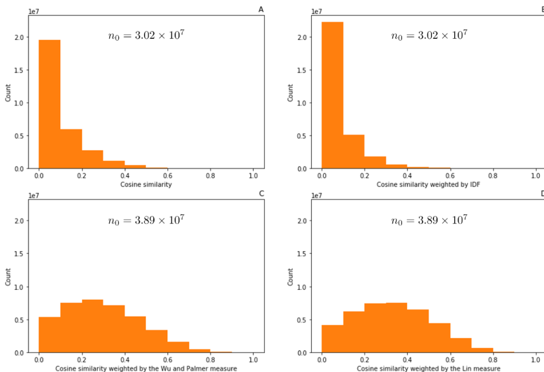
Figure 3: Similarity distributions in the female patient dataset
