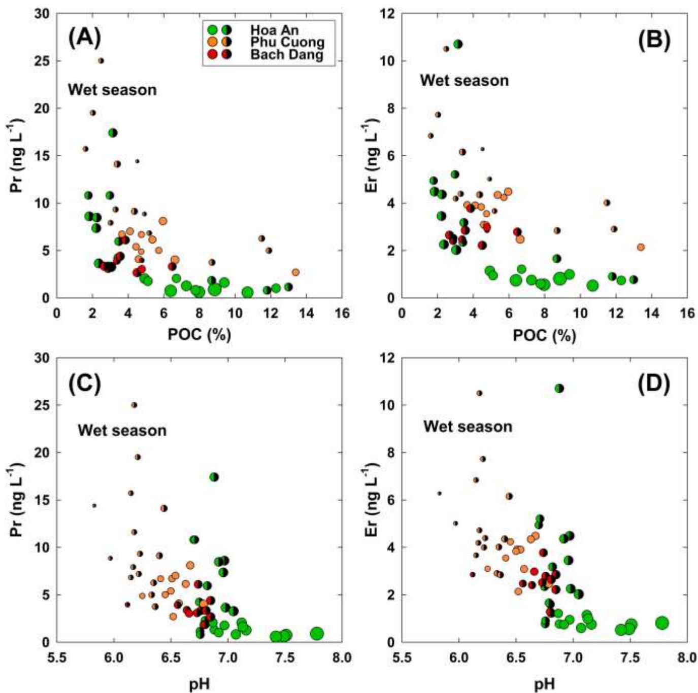
Fig. 3. The relationships of Pr and Er vs. particulate organic matter (A and B) and pH (C and D) at stations HA (green circles), PC (orange circles) and BD (red circles). The half-filled symbols show the samples taken during the wet season, while the open symbols represent the dry season samples. The symbol sizes in all four panels are proportional to pH values of the water samples (pH range from 5.83 to 7.78). (For interpretation of the references to colour in this figure legend, the reader is referred to the web version of this article.)
