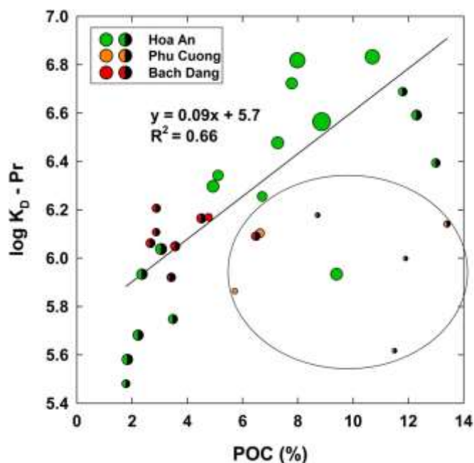
Fig. 7. The relationship between \log K_D of Pr and POC at stations HA (green circles), PC (orange circles) and BD (red circles). The half-filled symbols show the samples taken during the wet season, while the open symbols represent the dry season samples. The samples in the circles are excluded from the regression line. The symbol sizes are proportional to pH values of the water samples (pH range from 5.83 to 7.78). (For interpretation of the references to colour in this figure legend, the reader is referred to the web version of this article.)
