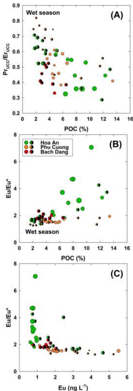
Fig. 4. The relationship between dissolved Pr/Er ratios (A) and Eu anomalies (B) with particulate organic carbon at stations HA (green circles), PC (orange circles) and BD (red circles). The half-filled symbols show the samples taken during the wet season, while the open symbols represent the dry season samples. Panel C shows the biplot of Eu anomalies as the function of dissolved Eu concentrations. The symbol sizes are proportional to pH values of the water samples (pH range from 5.83 to 7.78). (For interpretation of the references to colour in this figure legend, the reader is referred to the web version of this article.)
