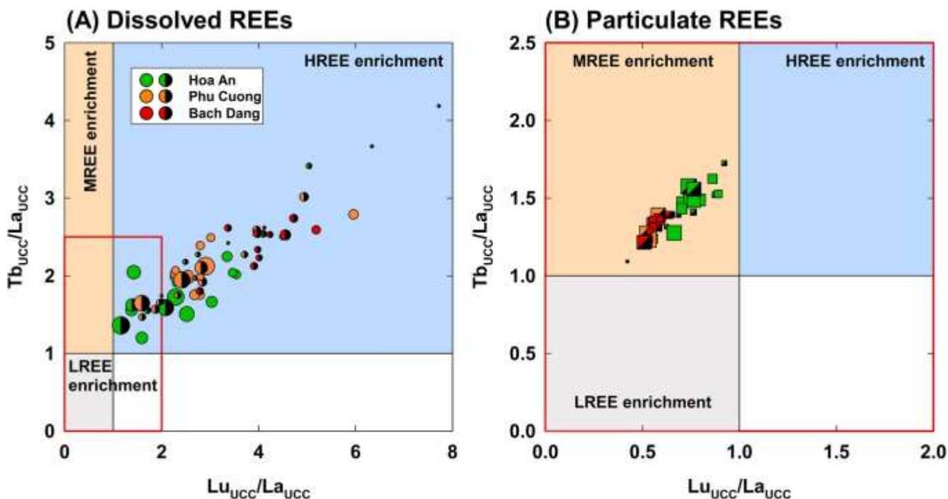
Fig. 5. Biplots of Tb_{UCC}/La_{UCC} as the function of Lu_{UCC}/La_{UCC} for dissolved (A) and particulate (B) fractions at stations HA (green circles), PC (orange circles) and BD (red circles). The half-filled symbols show the samples taken during the wet season, while the open symbols represent the dry season samples. The colored areas demark REE pattern types in environmental samples, i.e., the enrichment of LREEs, MREEs and HREEs. The symbol sizes are proportional to POC concentrations. (For interpretation of the references to colour in this figure legend, the reader is referred to the web version of this article.)
