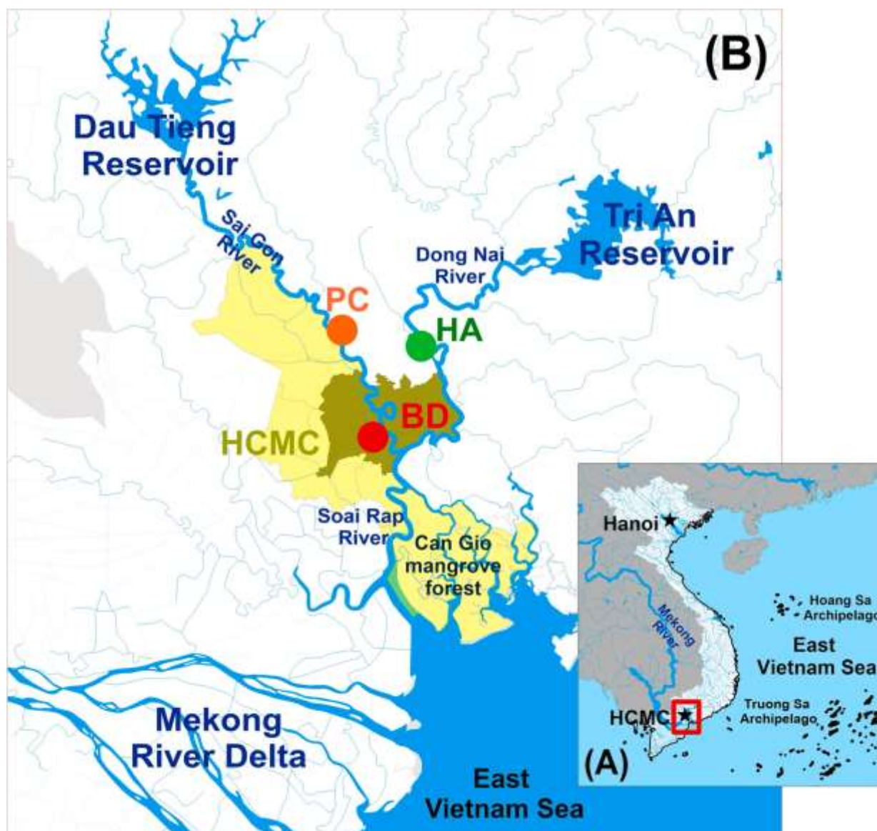
Fig. 1. Map of Vietnam (A) and the study region (B). The yellow area in B demarks Ho Chi Minh City (HCMC), while the dark yellow area shows the highly urbanized center of HCMC comprising sixteen urban districts. The three sampling stations include Phu Cuong (PC), Hoa An (HA) in the upstream sections of the Sai Gon and Dong Nai Rivers, respectively, and the urban station Bach Dang (BD) on the Sai Gon River. The dark blue lines show various river systems, and the fine blue straight lines highlight the dense canal systems of Southern Vietnam. (For interpretation of the references to colour in this figure legend, the reader is referred to the web version of this article.)
