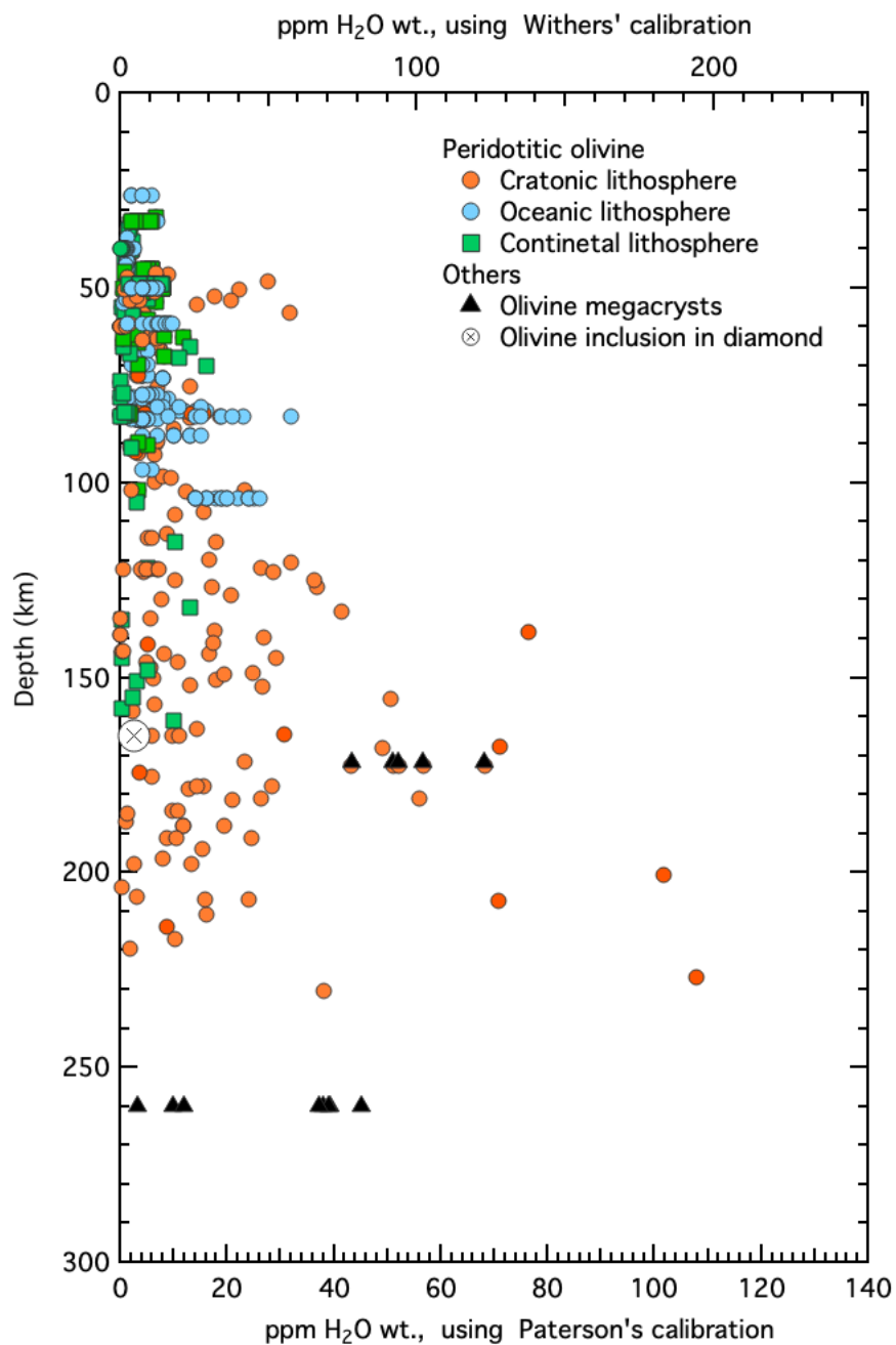
FIGURE 2. Hydrogen concentrations in olivine (in ppm wt H 2 O) as a function of depth for different geological contexts. UPDATED COMPILATION BASED ON DEMOUCY AND BOLFAN-CASANOVA (2016). Data source and methodology are provided in the online supplements.
