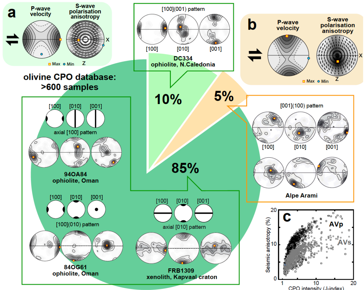
FIGURE 5. Pie chart showing the repartition of olivine CPO and seismic anisotropy patterns from the database of the Géosciences Montpellier EBSD facility, composed of > 600 peridotites including both peridotite massifs and peridotite xenoliths (Tommasi and Vauchez 2015). Olivine CPO and seismic anisotropy are displayed as pole figures, which are a stereographic representation of the orientation of lines and planes in 3D space. In all pole figures, the line marks the flow plane (Z is normal to the flow plane) and the flow direction (X) is E–W. Olivine CPO pole figures present the orientation of the three main crystallographic axes ([100], [010], and [001]) relative to the structural reference frame (here the flow plane and direction). Seismic anisotropy pole figures present the variation of P-wave velocity and the difference in velocity between the fast and slow quasi-S waves as greyscale colors. The polarization orientation of the fast quasi-S waves is indicated by white or black line segments for different propagation directions relative to the structural reference frame. (A) Typical seismic anisotropy pattern for olivine CPO formed by dominant [100] glide (green sections). (B) Typical seismic anisotropy pattern for olivine CPO formed by dominant [001] glide (orange section). (C) Maximum P- and S-wave anisotropies resulting from these olivine CPOs; variations in seismic anisotropy intensity result from variations
