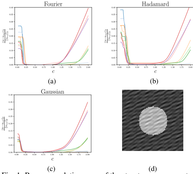
Fig. 1: Recovery relative error of the structure component with different gradient-sparsity s \in \{105, 139, 173\} and patch-rank r \in \{2, 4, 6\} via the LPR model with tuning parameters \mu = \frac{c}{\sqrt{s}} and \gamma = \frac{1}{\sqrt{r}} . (a) Fourier texture, (b) Hadamard basis and (c) Gaussian basis. (d) Example of a synthetic test image with a fourier texture used in this experiment.
