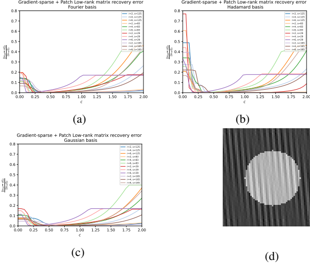
Fig. 1: Recovery relative error of the structure component with different gradient-sparsity s and patch-rank r via the LPR model with tuning parameters \mu = \frac{c}{\sqrt{s}} and \gamma = \frac{1}{\sqrt{r}} . (a) Fourier texture, (b) Hadamard, (c) Gaussian basis, (d) Example of a synthetic test image.
